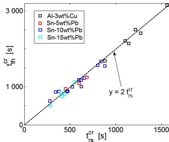
Figure 32: The thermal ( t_{th} ) and the tip response time ( t_{rs} ) at the CF corresponding to the beginning of the oscillatory evolution of the CF
