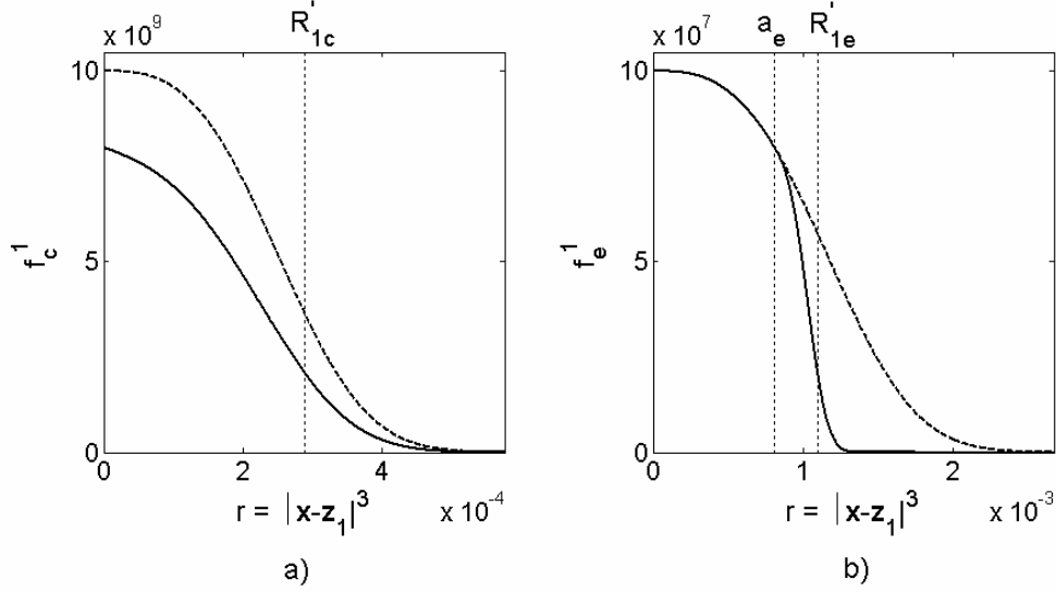
Figure 12: The nearest columnar (a) and equiaxed (b) neighbor distribution before (dashed line) and after (full line) the c/e coexistence ( a_e = 810 \mu\text{m} , n_e = 10^8 \text{ grains/m}^3 and n_c = 10^{10} \text{ grains/m}^3 )
