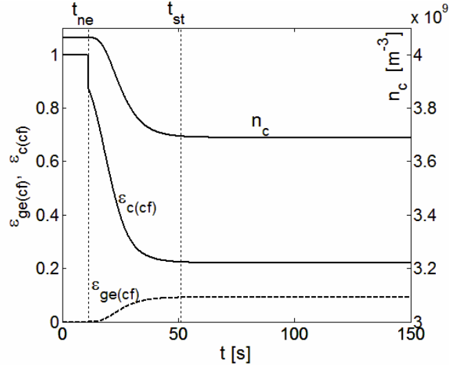
Figure 13: The evolution of the equiaxed grain fraction, the columnar fraction and the columnar grain density at the CF (Al-3wt%Cu, CR = 0.1 K/s, \Delta T_{ne} = 1K , n_e = 10^9 m -3 , V_p = 8 \cdot 10^{-5} m/s, no first mechanical blockage effect)
