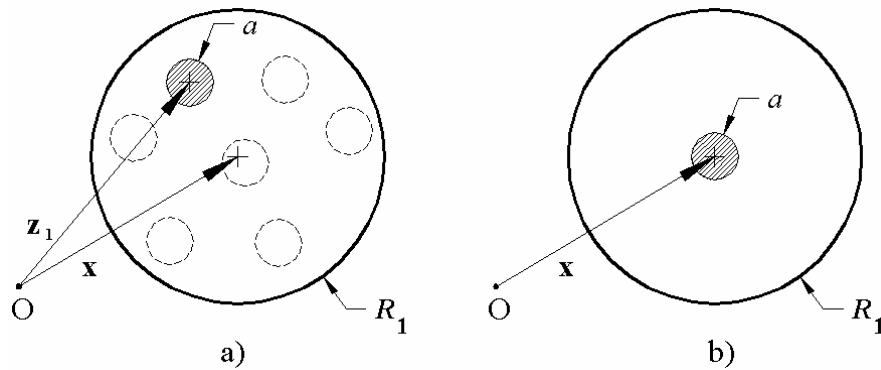
Figure 5: a) The cell approximation to the ensemble average; b) The cell approximation to the volume average
