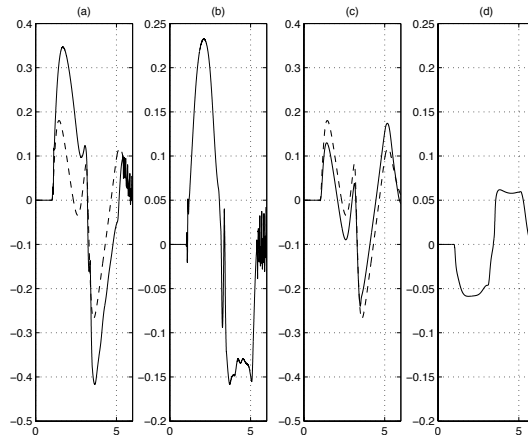
Figure 5.3: STC (5.13) with nominal parameters: a) \omega_z (solid) and \omega_{z,\text{ref}} (dashed) [rad/s vs s]; b) Tracking error e = \omega_z - \omega_{z,\text{ref}} . STC (5.13) with parametric estimation (5.19): c) \omega_z [rad/s vs s]; d) Tracking error e = \omega_z - \omega_{z,\text{ref}} .
