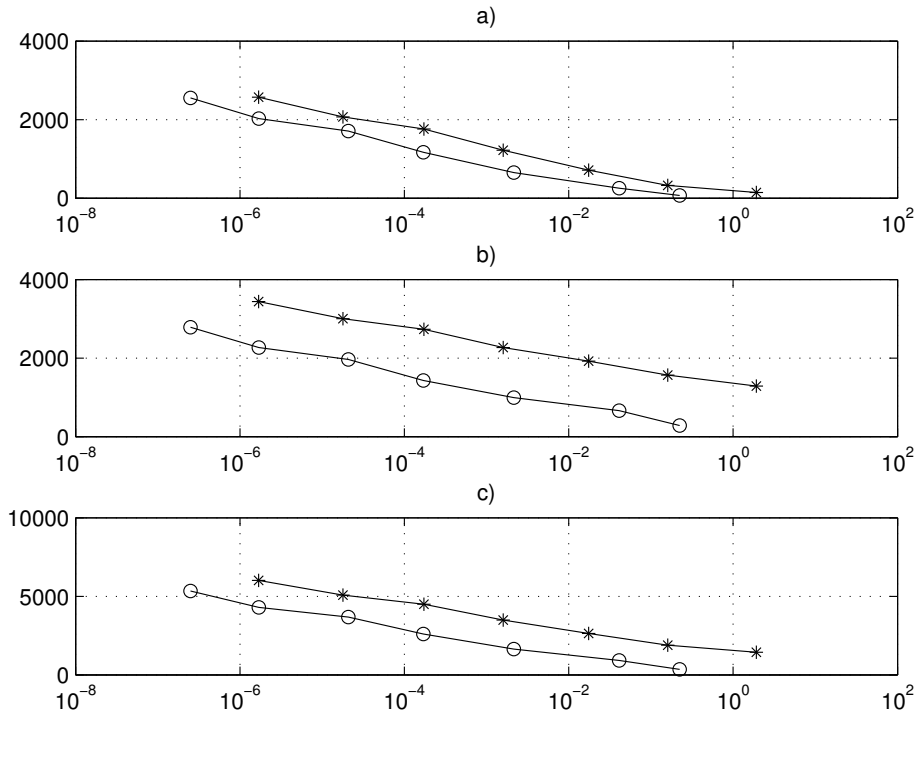
Figure 2.13: Controller based on the impulsive observer (2.36) (circle) and Luenberger-like observer (2.45) (star) with \tau_{\max}^s = \tau_{\ell}^s = 0.3 s and \tau_{\max}^a = \tau_{\ell}^a = \infty : a) Number N_s of sensor communications versus stabilization error norm \|x\|_{ss} ; b) Number N_a of controller communications versus stabilization error norm \|x\|_{ss} ; c) Number N_s + N_a of sensor and controller communications versus stabilization error norm \|x\|_{ss} .
