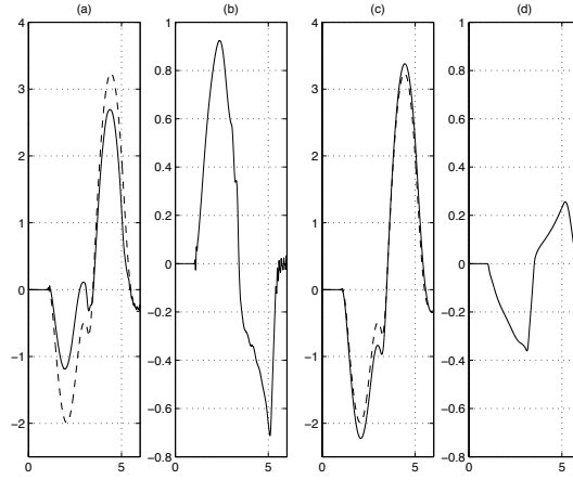
Figure 5.2: STC (5.13) with nominal parameters: a) v_y (solid) and reference v_{y,\text{ref}} (dashed) [m/s vs s]; b) Tracking error e = v_y - v_{y,\text{ref}} . STC (5.13) with parametric estimation (5.19): c) v_y (solid) and reference v_{y,\text{ref}} (dashed) [m/s vs s]; d) Tracking error e = v_y - v_{y,\text{ref}} .
