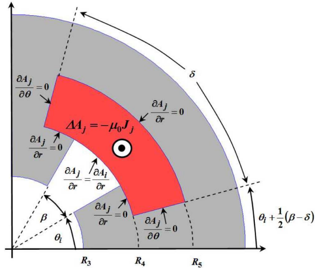
Fig. 3. j th slot subdomain with its boundary conditions (with homogeneous current density J_j in the slot).
