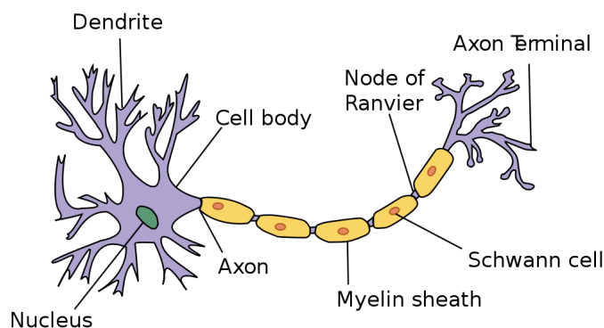
Figure 3.1.: Neuron structure.
