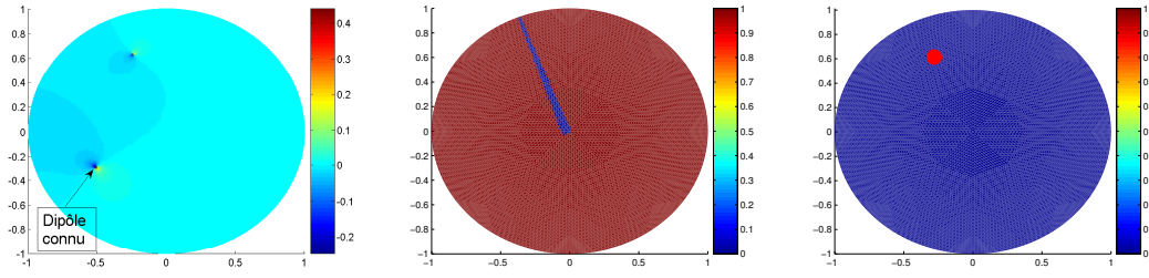
Figure 3.11.: From left to right, known and unknown dipolar sources, cone of the potential solutions, localisation of the unknown dipolar source.
