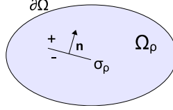
Figure 2.9.: Cracked domain.
