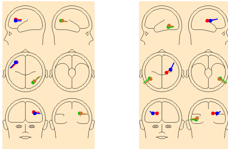
Figure 3.16.: Two results with two dipolar sources and a rms noise of 20\mu v .
