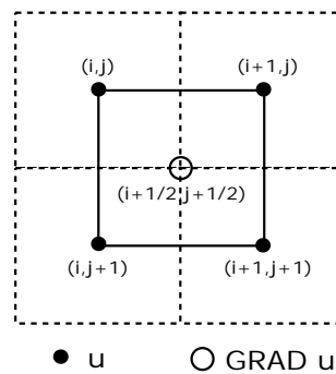
Figure A.1.: Stencil for operator GRAD.
