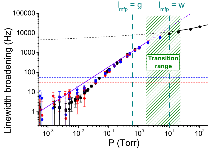
Figure V.14: Evolution of the linewidth for the 100 \mu\text{m} device modes as a function of the pressure in the cell. We focus here on the low pressure data, where the mean-free-path becomes larger than the width of the beam, which is then described as the molecular regime (purple line). We could measure in this range the three modes introduced in Fig. V.12 (same conventions), and observe a similar behaviour for each of them. However, when l_{mfp} is larger than the gap g between the bottom of the chip and the beam, we observe a clear deviation between the experimental data and the calculation. The dashed horizontal lines represent the linewidth of each mode in vacuum, which gives an idea of the subtractions involved to capture the broadening of the linewidths and which cannot explain the deviation.
