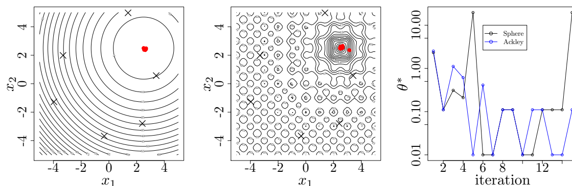
Figure 6.5: DoEs created by the toy greedy algorithm 6.1 after 15 iterations on the Sphere (left) and the Ackley (middle) functions. Right: plot of “best” length-scale, \theta^* . \theta^* oscillates during optimization iterations and usually has a small magnitude after the first iterations. The y-axis is in logarithmic scale.
