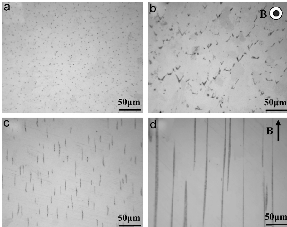
Fig. 4. Microstructure of MnBi/Bi eutectic solidified at 5 μm/s without and with the magnetic field (a) 0 T, transverse section; (b) 10 T, transverse section; (c) 0 T, longitudinal section; (d) 10 T, longitudinal section.
