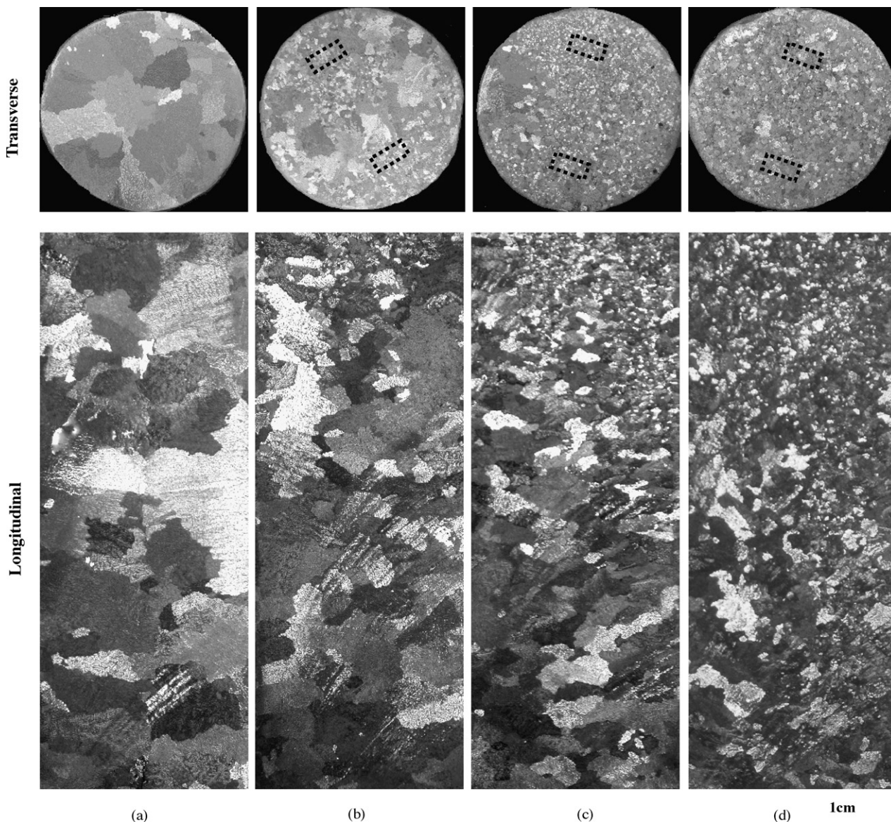
Fig. 6. Effect of the electromagnetic force on the structures under the gradient magnetic field of B = 10\text{ T} , B_z \text{ dB}_z/\text{dz} = 400\text{ T}^2/\text{m} : (a) I = 0\text{ A} ; (b) I = 1\text{ A} ; (c) I = 3\text{ A} ; (d) I = 10\text{ A} .
