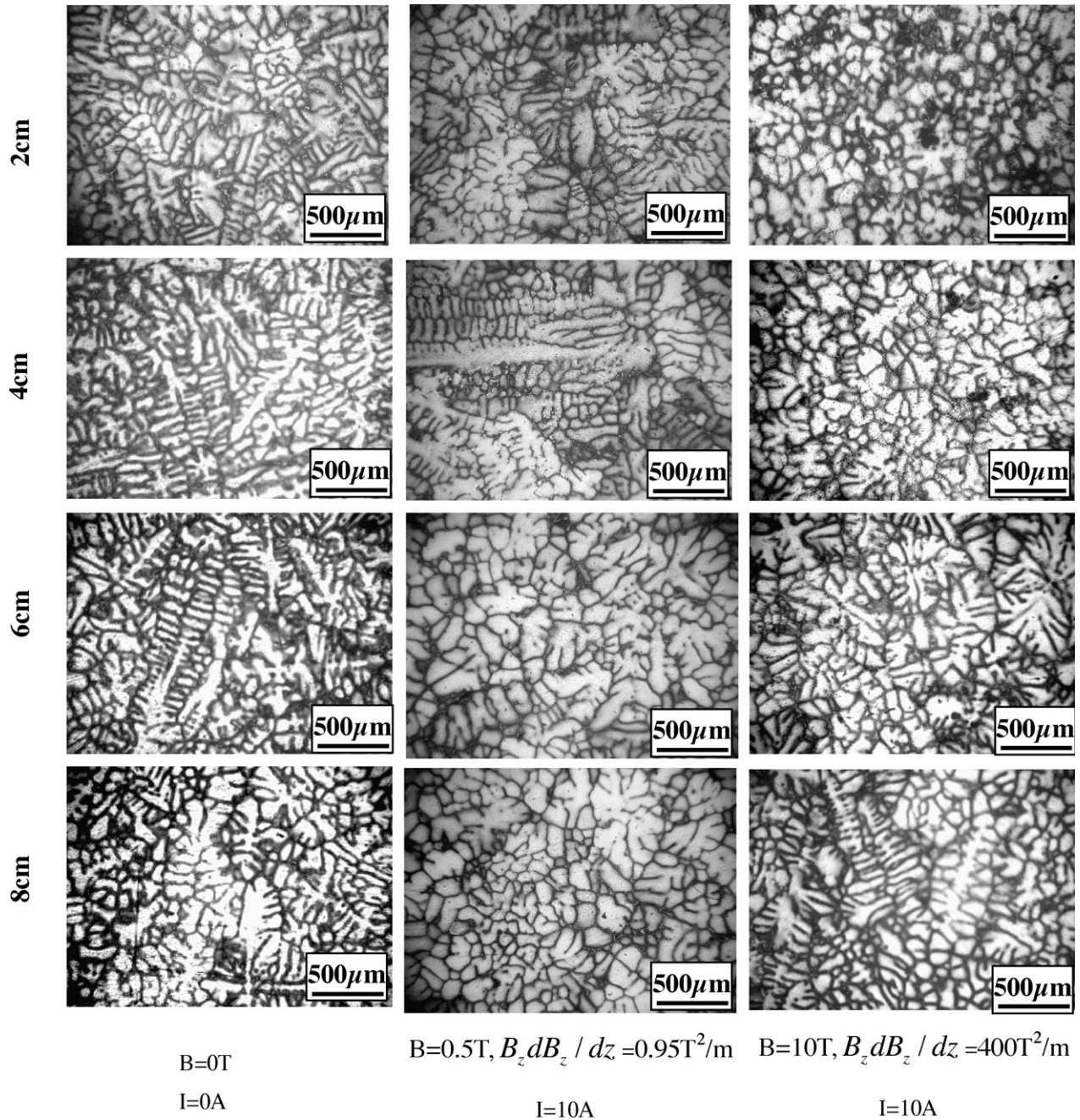
Fig. 11. Effect of the simultaneous imposition of electromagnetic and magnetic forces on the microstructure of Al–4.5 wt.%Cu alloy at various positions from the electric poles.
