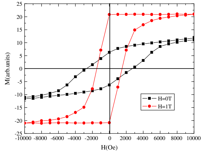
Fig. 5. Hysteresis loops of samples solidified at 0 T and 1 T which are measured along the fabrication field H_f .
