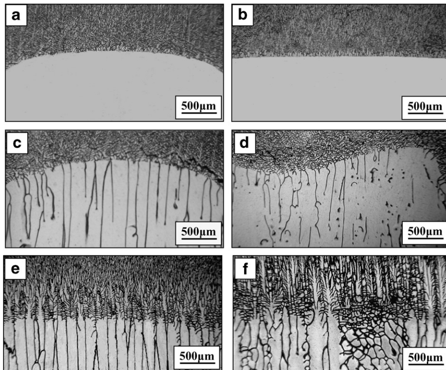
Fig. 4. Longitudinal structures of an Al-0.85 wt.%Cu alloy and the quenched liquid–solid interface for various growing velocities: (a) 0 T, 0.5 \mu\text{m s}^{-1} ; (b) 10 T, 0.5 \mu\text{m s}^{-1} ; (c) 0 T, 2.5 \mu\text{m s}^{-1} ; (d) 10 T, 2.5 \mu\text{m s}^{-1} ; (e) 0 T, 20 \mu\text{m s}^{-1} ; (f) 10 T, 20 \mu\text{m s}^{-1} .
