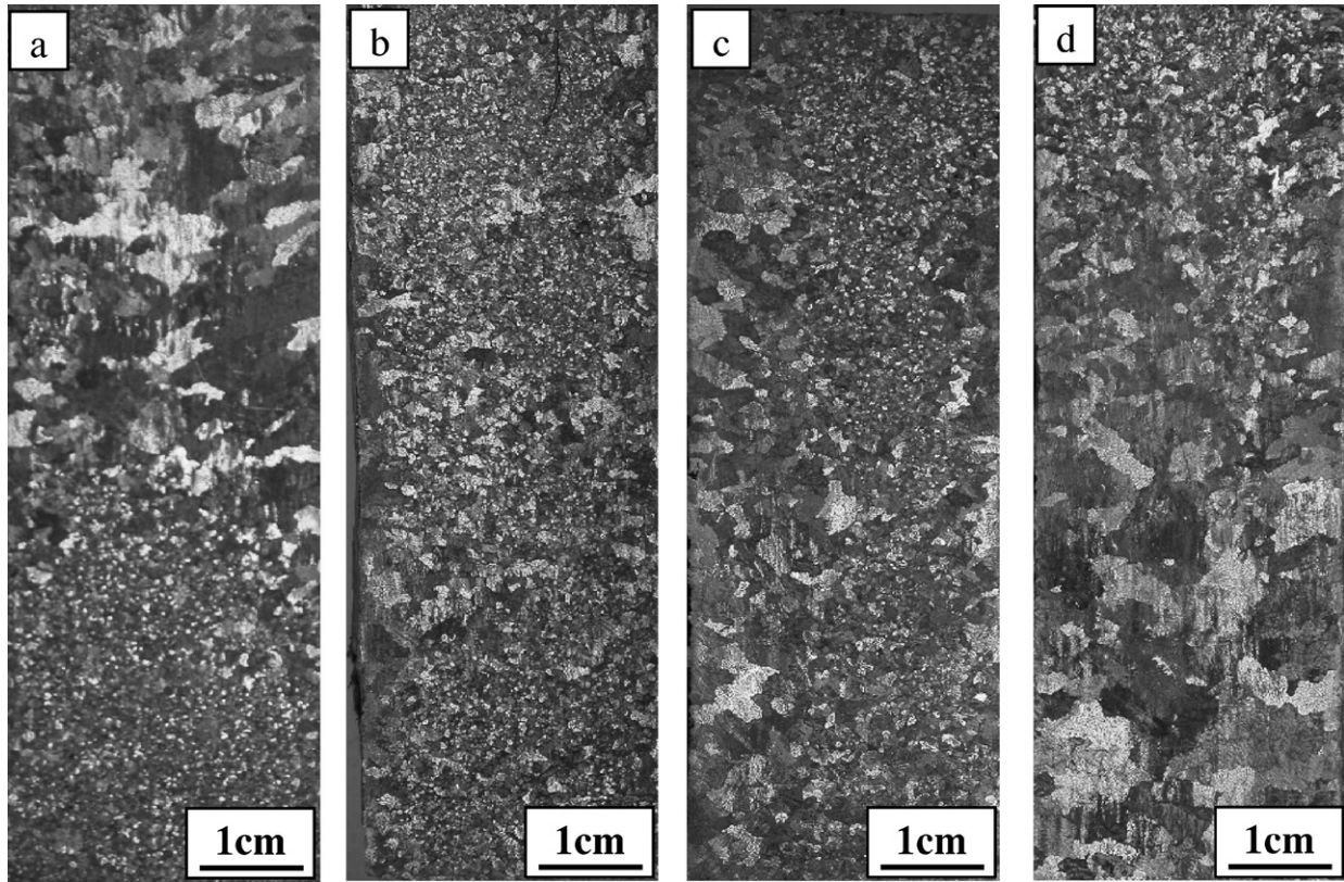
Fig. 4. Effects of a magnetic force on the structures of pure Al at the same electromagnetic force density: (a) B = 0.5 T and B_z dB_z/dz = 0.95 T 2 /m, I = 20 A; (b) B = 1.5 T and B_z dB_z/dz = 8.5 T 2 /m, I = 6.5 A; (c) B = 2 T and B_z dB_z/dz = 16.2 T 2 /m, I = 5 A; (d) B = 6 T and B_z dB_z/dz = 150 T 2 /m, I = 1.6 A.
