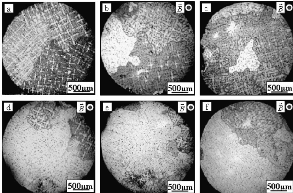
Fig. 14. The columnar-to-equiaxed transition as a function of the magnetic field intensity in directionally solidified the Al-4.5 wt.%Cu alloy at a growth speed of 20 \mu\text{m/s} and a temperature gradient of 62.8°C/cm: (a) 0 T, (b) 2 T, (c) 4 T, (d) 6 T, (e) 8 T and (f) 10 T.
