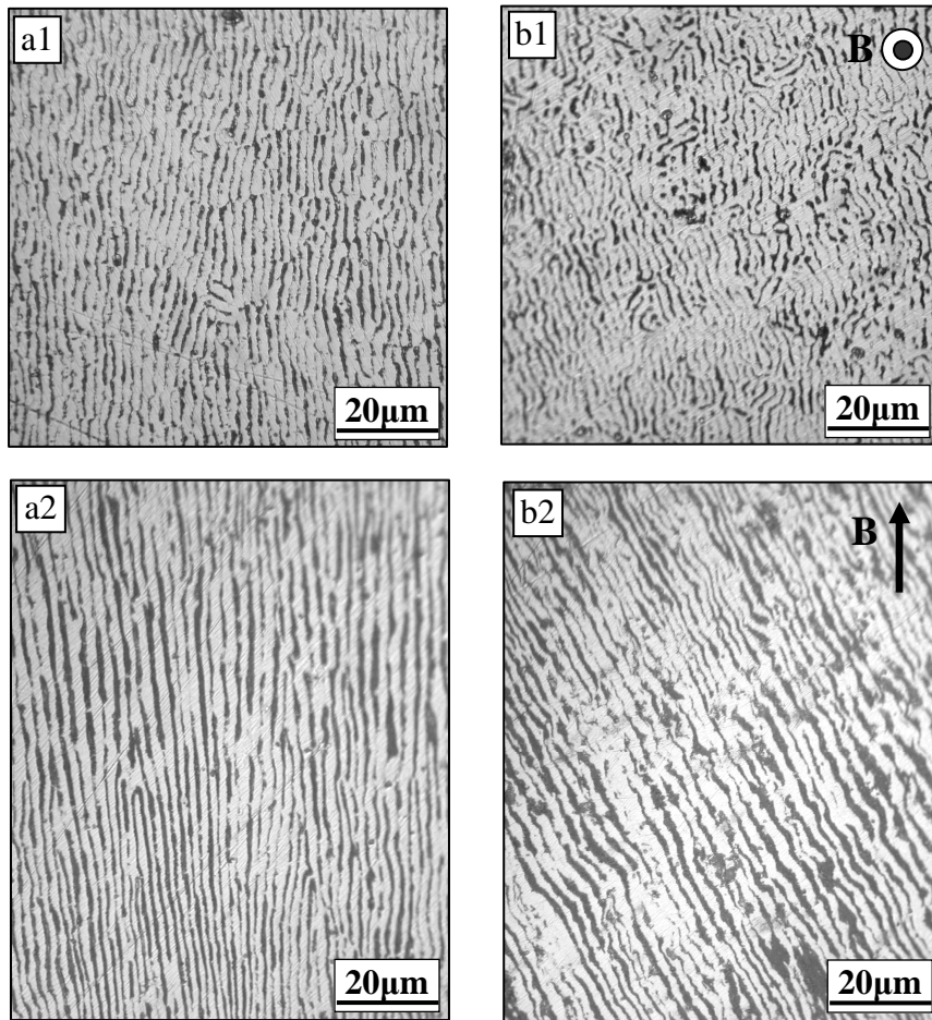
Fig. 4.2. Microstructures in directionally solidified Pb-Sn eutectic alloy without (a) and with a 10T magnetic field (b) ( G_L=45\text{K}/\text{cm} , R=2\mu\text{m}/\text{s} ) .
