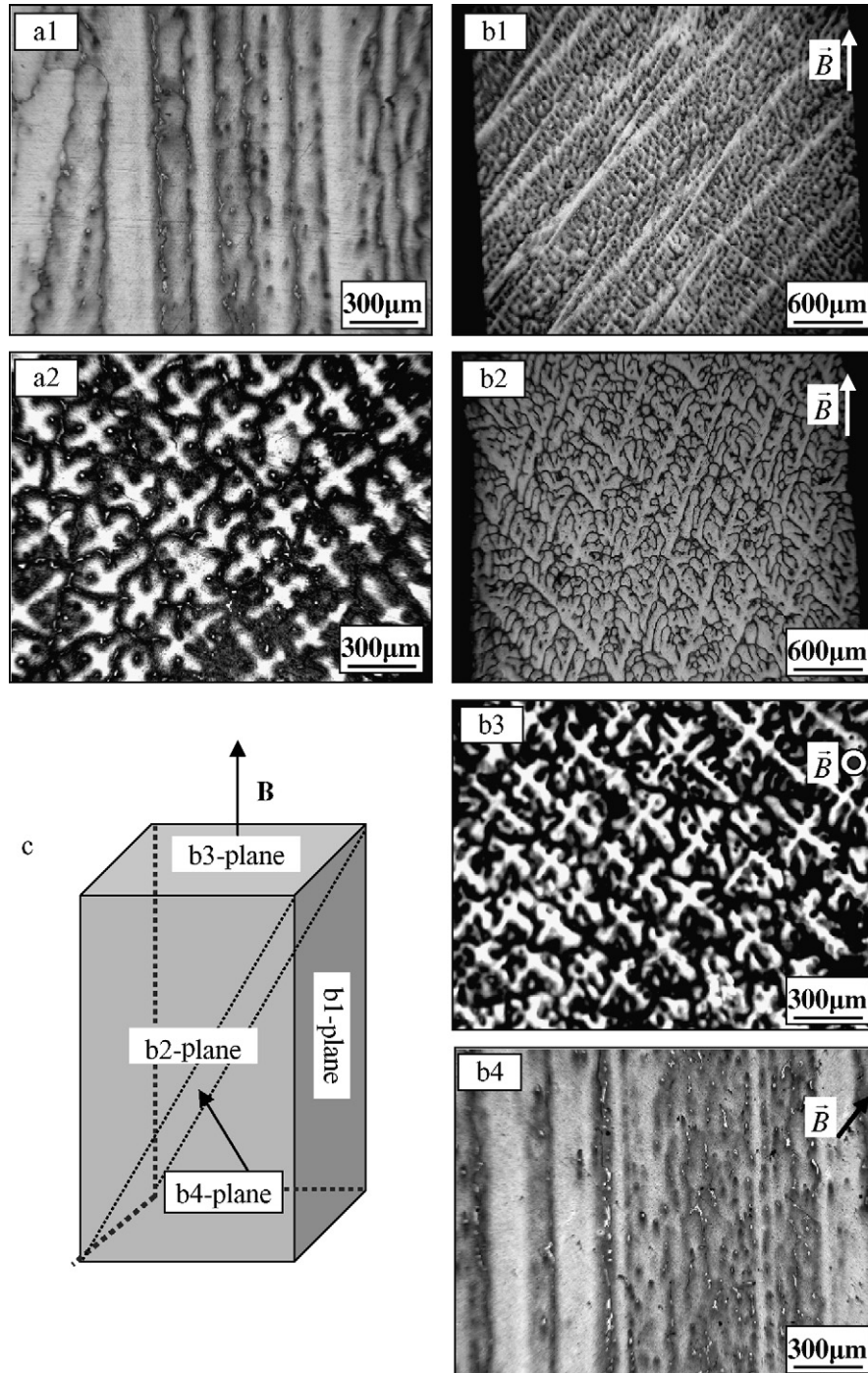
Fig. 5. Microstructures in directionally solidified the Al-4.5 wt.%Cu alloy at a growth speed of 50 \mu\text{m/s} and a temperature gradient of 38 \text{ }^\circ\text{C/cm} (a) without and (b) with a 10 T-magnetic field: (a1) Longitudinal microstructure; (a2) transverse microstructure; (b1) longitudinal microstructure; (b2) longitudinal microstructure; (b3) transverse microstructure; (b4) microstructure along the direction angled 45^\circ with the solidification direction and (c) schematic view of incising sample.
