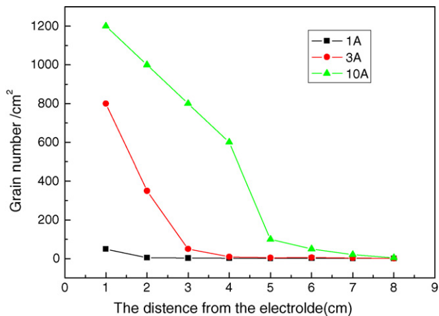
Fig. 9. The grains number on the longitudinal section as a function of the distance from the electrode under a gradient magnetic field of B = 10 T, B_z dB_z/dz = 400 T 2 /m and various current intensities.
