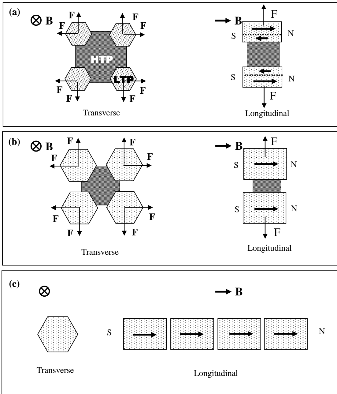
Fig. 17. Schematic illustration of the Mn_{1.08}Bi -to- MnBi phase transformation process in the magnetic field.
