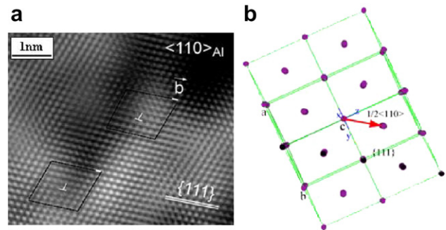
Figure 6. HREM image of the Al lamellar in Figure 5(b1) and the dislocation schematic map. (a) The HREM image on the {111}-crystal plane; (b) the schematic map of the dislocation analyses.
