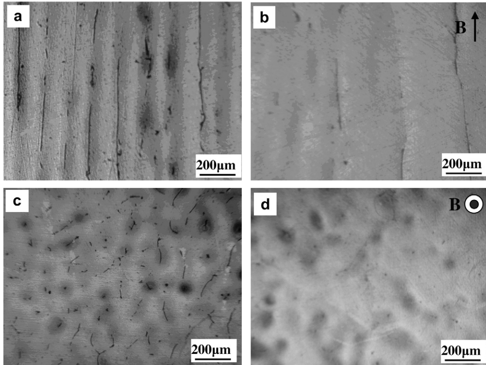
Fig. 5. Microstructures below the eutectic isotherm of Al-0.85 wt.% Cu alloy solidified at 10 µm/s and a temperature gradient in liquid ( G_L ) of 62.8 K/cm. (a) Longitudinal, 0 T; (b) longitudinal, 10 T; (c) transverse, 0 T; and (d) transverse, 10 T.
