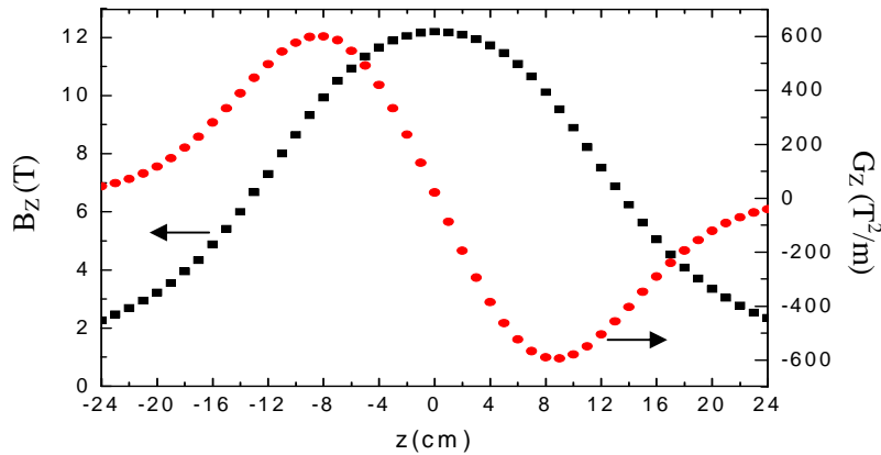
Fig. 2. Field profiles in the magnetic field operating at 12T. B_z is the vertical component of the field on the axis of the coil. G_z is the vertical component of \text{grad}(B_z^2/2) on the axis of the coil (i.e. B_z dB_z / dz ), z is the distance above the coil.
