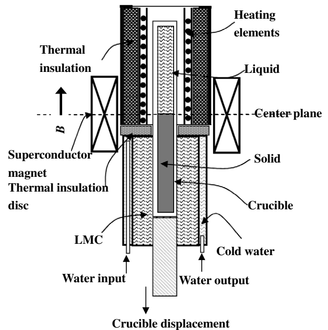
Fig. 1. Schematic illustration of the Bridgman solidification apparatus in a superconducting magnet.
