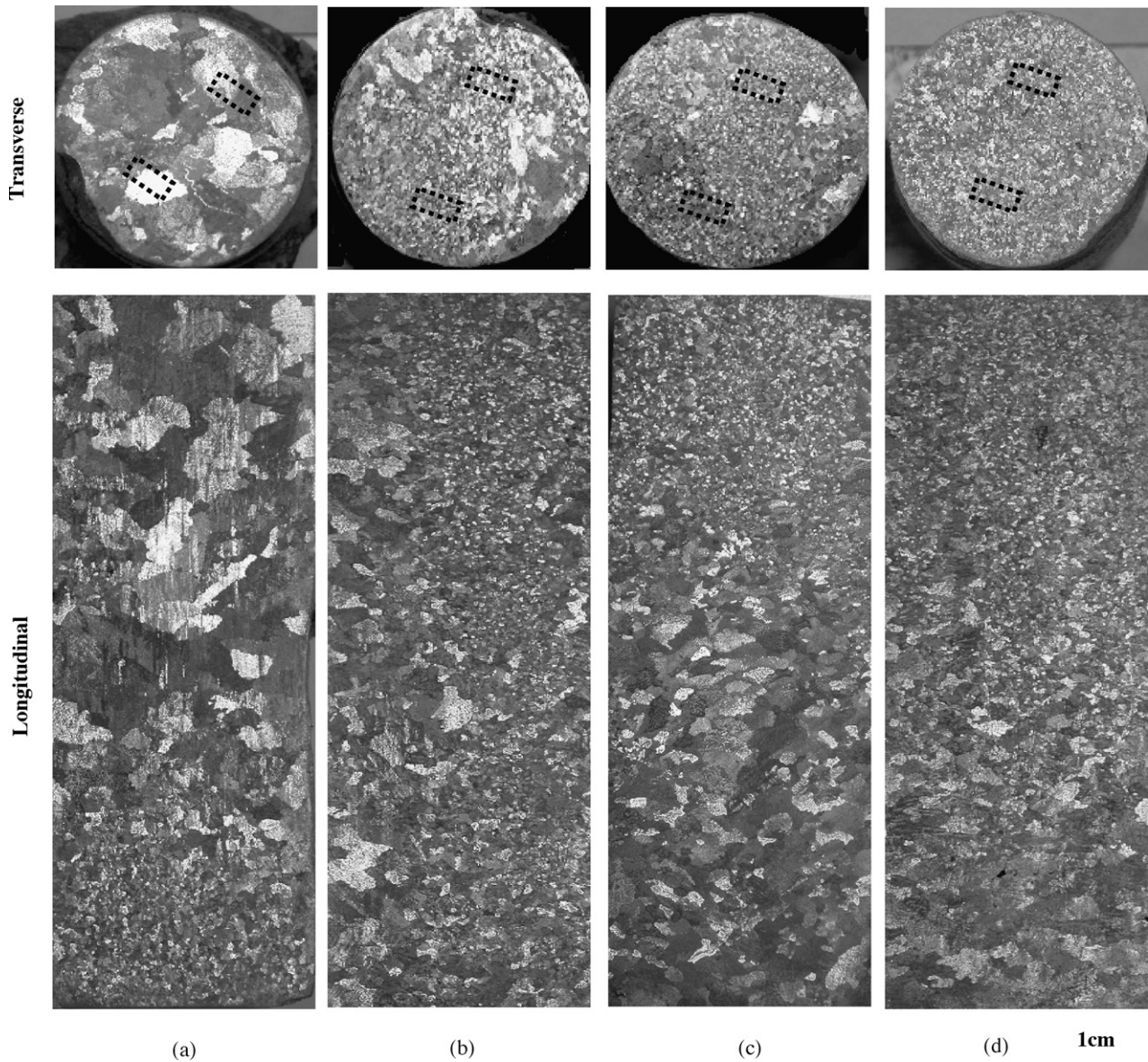
Fig. 7. Effect of the electromagnetic and magnetic forces on the structures under the same electric current density of 10 A with the frequency of 50 Hz (a) B = 0.8 T and B_z dB_z/dz = 6.4 \text{ T}^2/\text{m} , I = 10 A; (b) B = 2 T and B_z dB_z/dz = 16.2 \text{ T}^2/\text{m} , I = 10 A; (c) B = 4 T and B_z dB_z/dz = 64.4 \text{ T}^2/\text{m} , I = 10 A; (d) B = 8 T and B_z dB_z/dz = 244.6 \text{ T}^2/\text{m} , I = 10 A.
