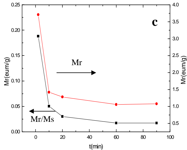
Fig. 14. The magnetic properties of the same sample as shown in Fig. 7.
