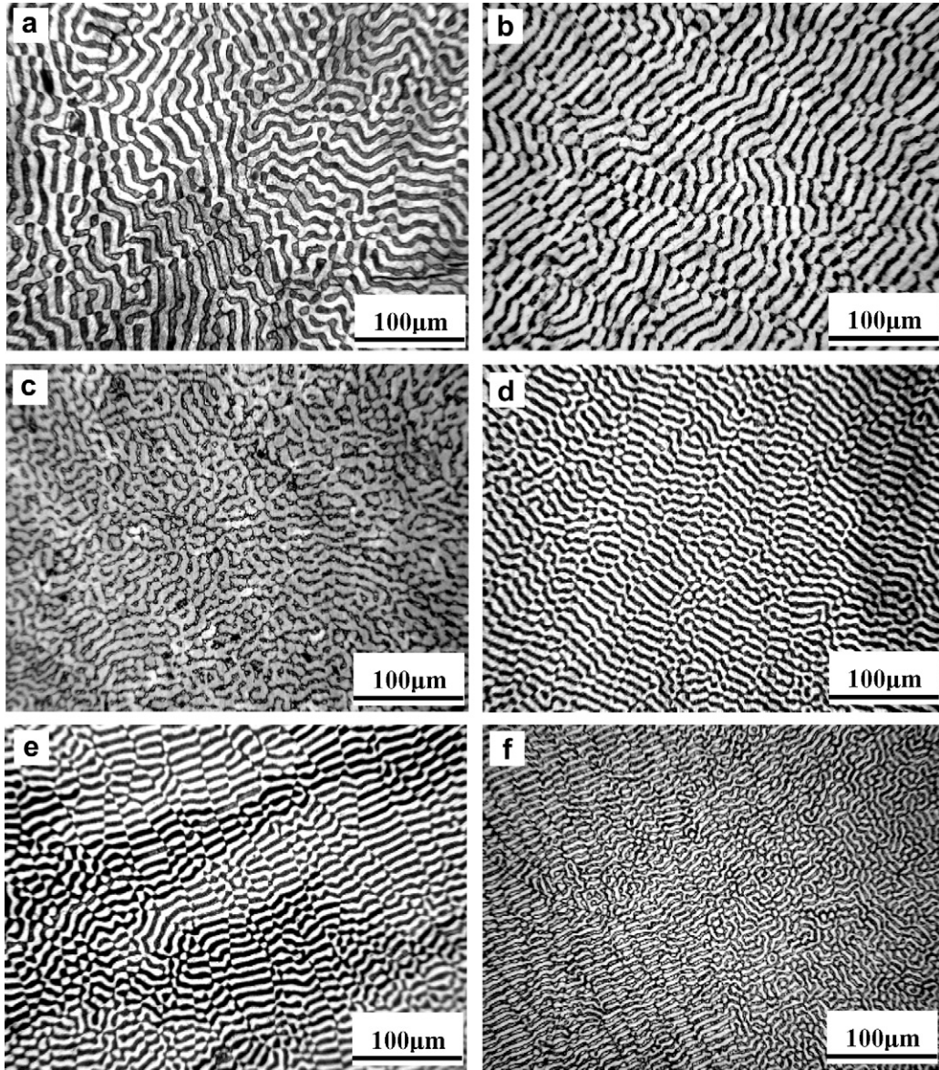
Fig. 7. Transverse microstructures of the samples directionally solidified at 0.5 \mu\text{m/s} in various magnetic field intensities. (a) B = 2\text{ T} , (b) B = 3\text{ T} , (c) B = 4\text{ T} , (d) B = 6\text{ T} , (e) B = 8\text{ T} and (f) B = 10\text{ T} .
