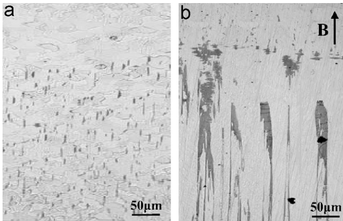
Fig. 3. The microstructure at the solid/liquid interface solidified at 2 μm/s without the field (a) and with a 10 T field (b).
