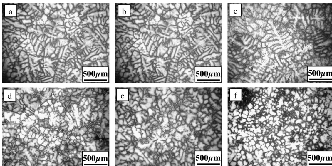
Fig. 10. Effect of an electromagnetic force on the solidification microstructure of Al–4.5 wt.%Cu alloy on the transverse section at the position 2 mm from the electric poles: (a) B = 0 T, I = 0 A; (b) B = 0 T, I = 10 A; (c) B = 10 T, I = 0 A; (d) B = 10 T, I = 1 A; (e) B = 10 T, I = 5 A; (f) B = 10 T, I = 10 A.
