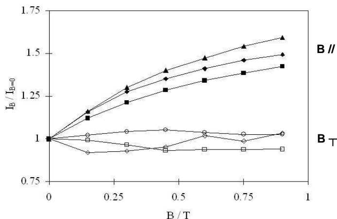
Figure 2.4. Rapport I_B/I_{B=0} , en fonction du champ B , Electrode Ag(0,2\text{ cm}^2) . L. Rabah et al. [72] 1). B // ; ( \blacktriangle ) 100 mV; ( \blacklozenge ) 80 mV; ( \blacksquare ) 65 mV. 2). B \perp ; ( \diamond ) 80 mV; ( \square ) 65 mV; ( \circ ) 50 mV
