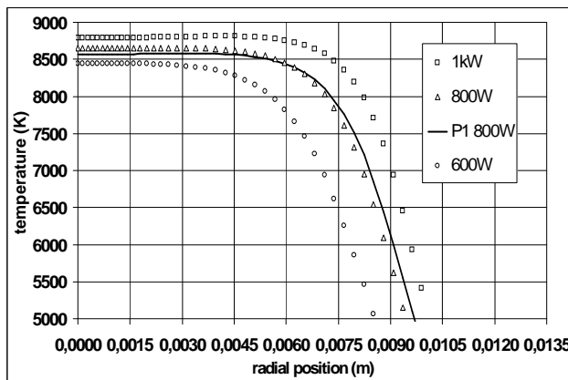
Figure 7: Temperature simulated along a plasma radius at z=-5,5mm.
