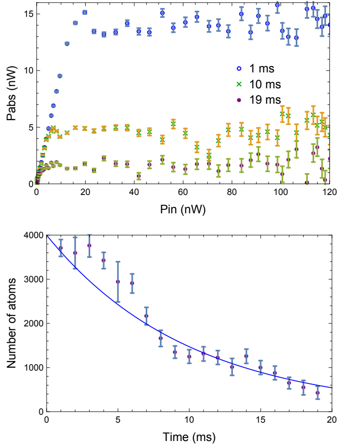
Figure 4.13: Top: Saturation of the absorbed power from a probe resonant on \{6S_{1/2}, F = 4\} \rightarrow \{6P_{3/2}, F = 5\} . The absorbed power ( P_{in}-P_{out} ) is given as a function of the input power. Bottom: Number of atoms derived with Eq. (2.3.1) as a function of time. The blue curve corresponds to an exponential decay with a 10 ms time constant.
