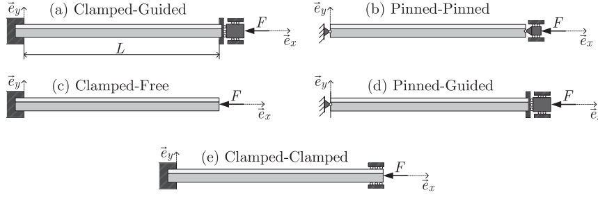
Fig. 2. Boundary conditions.
