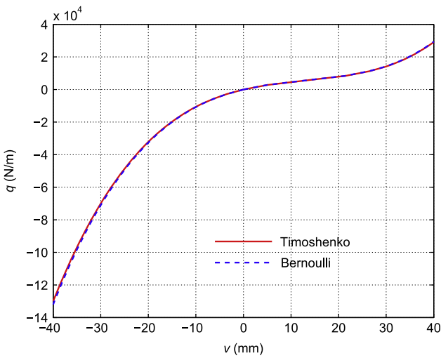
Fig. 9. Example 2: non-linear response for h=0.05 \text{ m} .
