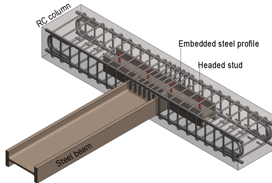
Figure. 2. New RCS connection detail.
