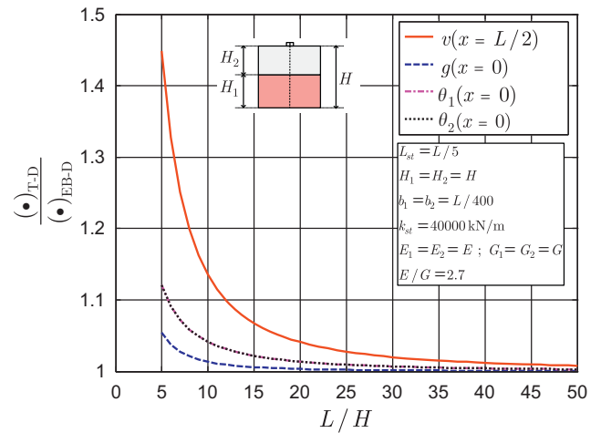
Fig. 14. Influence of length–dept ratio on the deflection, the slip and the rotations.
