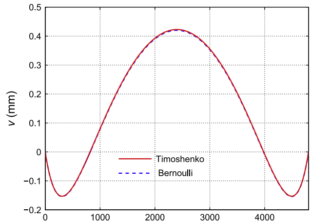
Fig. 12. Example 3: deflection pattern for the slender beam.
