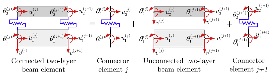
Fig. 4. Illustration of the two-layer beam finite element.
