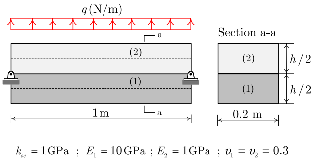
Fig. 8. Example 2: non-linear response of pinned laminated beam.
