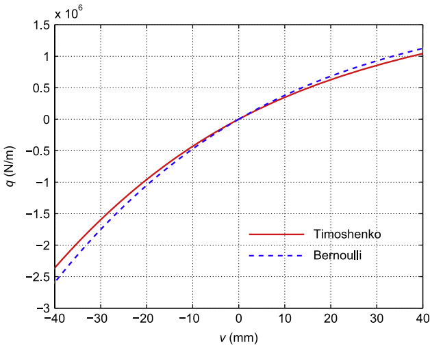
Fig. 10. Example 2: non-linear response for h=0.2 \text{ m} .
