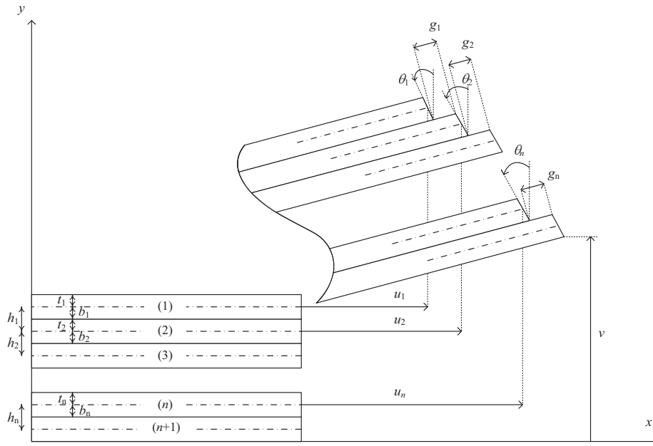
Fig. 1. Displacement field of a multi-layered beam.
