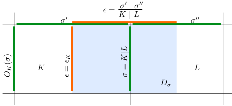
FIGURE 3.2 – Notations for the dual mesh.
