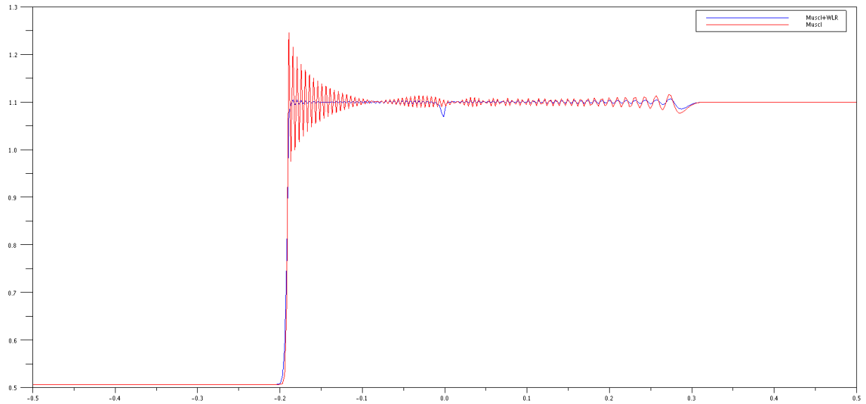
FIGURE 2.11 – Configuration 4 – Density – Cutline at y = 0.48 – Solution without artificial viscosity in red and with WLR viscosity in blue.
