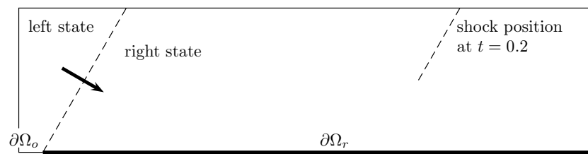
FIGURE 2.13 – Double Mach reflection – Geometry and initial conditions.
