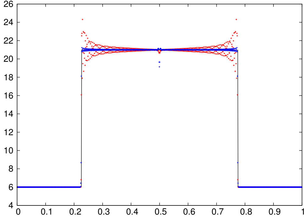
FIGURE 2.7 – A 1D Riemann problem : the "symetrical double shock" – h = 0.001 and \delta t = h/60 – Density at t = 0.035 . Upwind solution without (red) and with (blue) WLR viscosity
