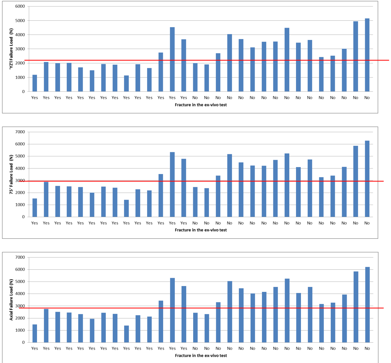
Figure 3-15 : Evaluation of the ratio Failure Load over the fractured and non-fractured cases at the first impact of the ex-vivo experiment Chapter 2. This figure presents the results for 1) Top: the model 'YZ' (-45°), 2) Middle: the fall case model (75°) and 3) Bottom: the axial model (standart HR-pQCT).
