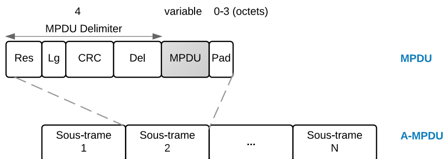
Figure 1.9 – Format A-MPDU
