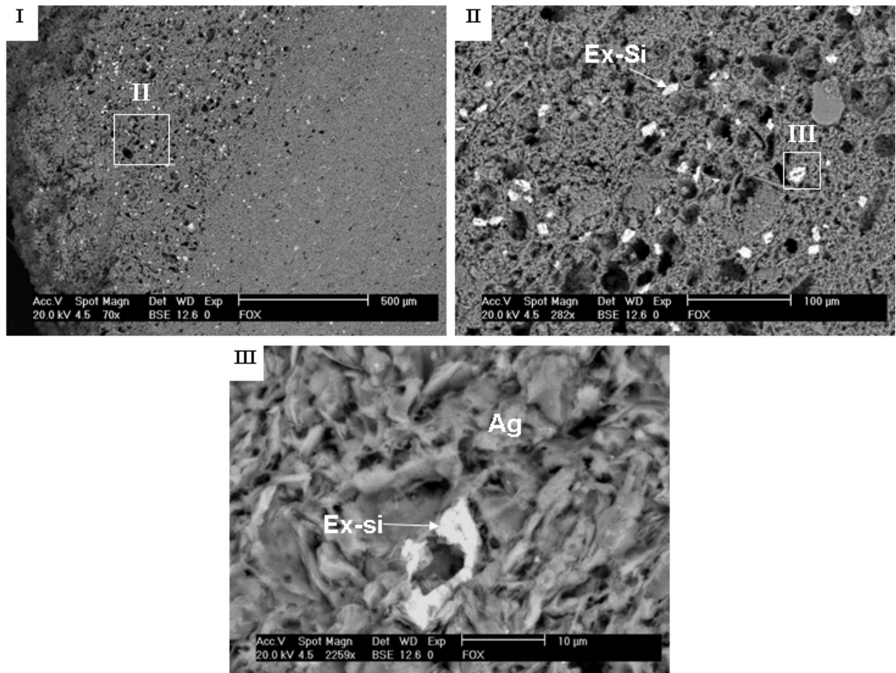
Figure 3-21 : SEM backscattered images of the caprock sample after experiment with NO and saline water (25 g/l). (I) global view; (II and III) successive zooms on the matrix. (Ex-Si) ex-siderite transformed in hematite, (Ag) clay minerals.
