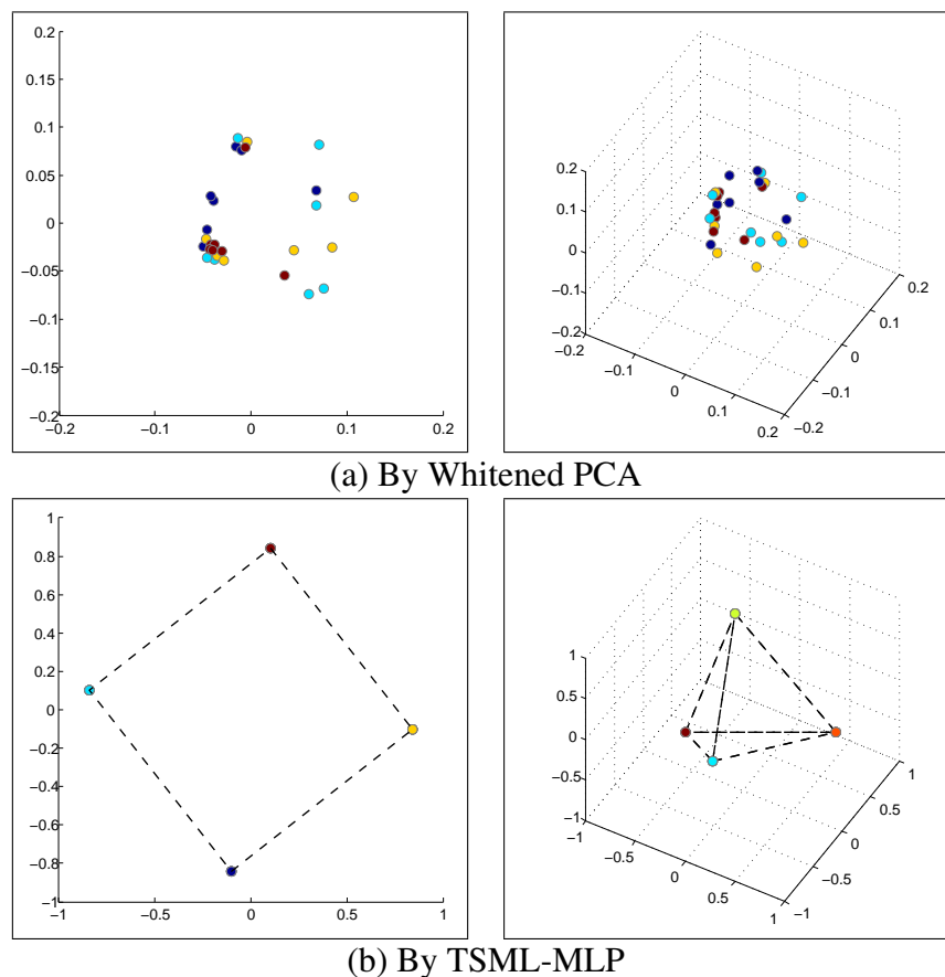
Fig. 5.6 Visualization of dimensionality reduction into the 2-d or 3-d spaces using (a) Whitened PCA and (b) TSML-MLP.
