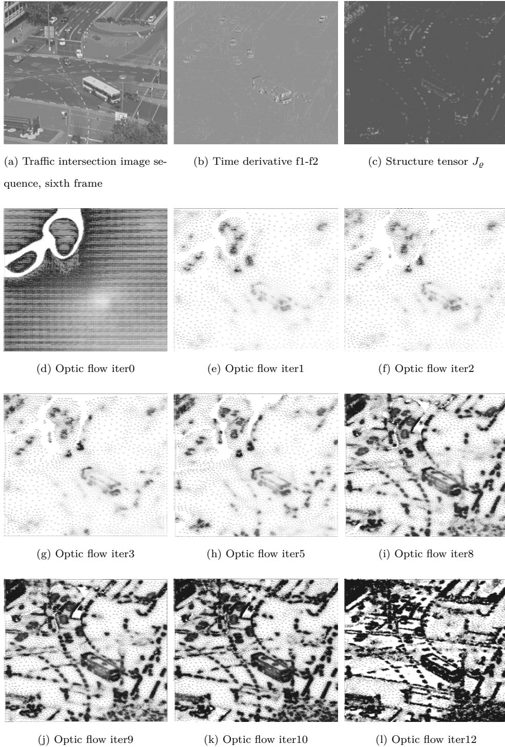
Figure 5.13: Traffic intersection image sequence and TV regularization with improved data term.
