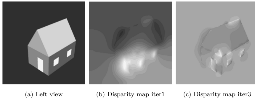
Figure 4.16: TV Regularization For House Stereo Pair
