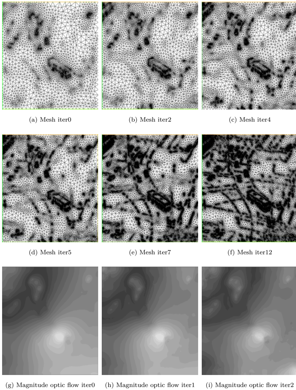
Figure 5.14: Traffic intersection image sequence and TV regularization with improved data term.
