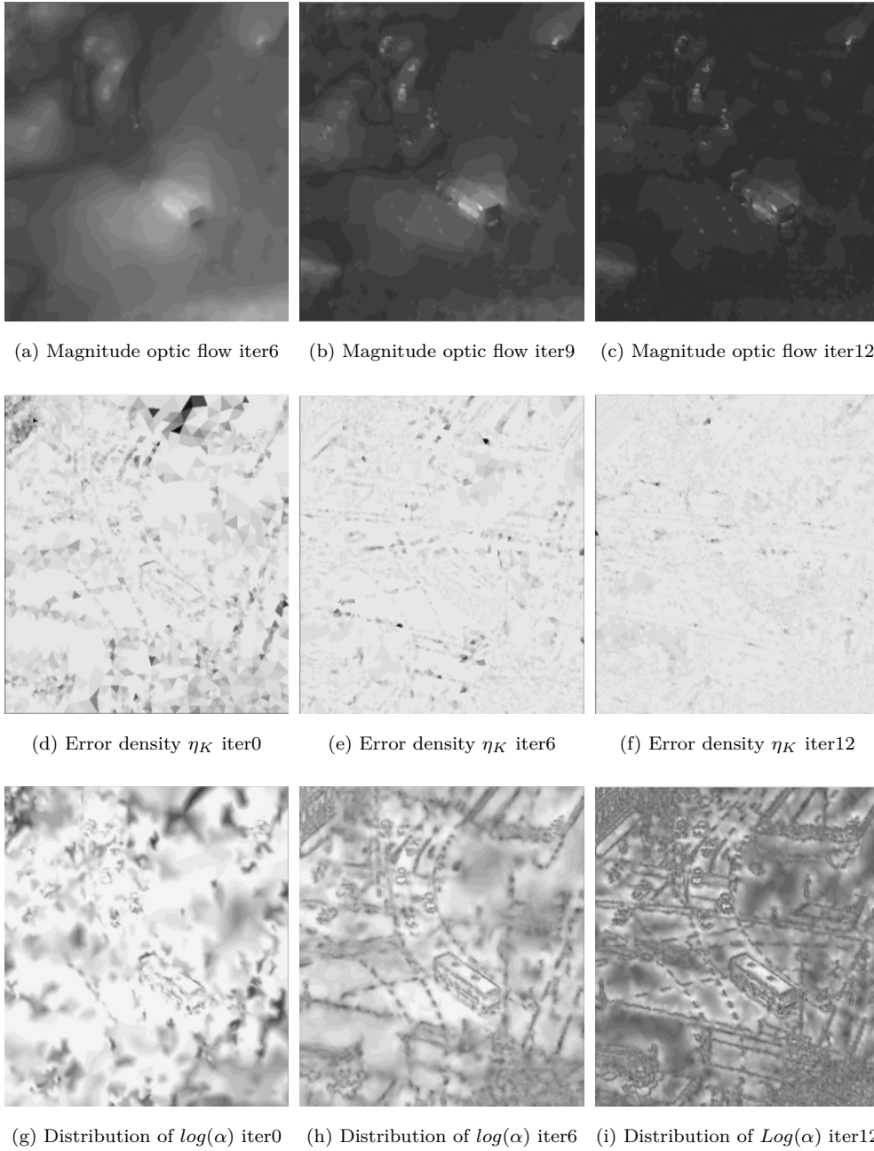
Figure 5.15: Traffic intersection image sequence and TV regularization with improved data term.
