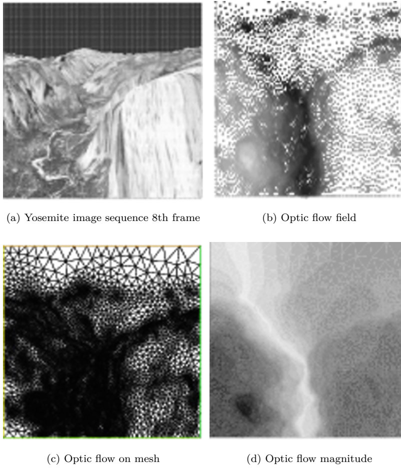
Figure 1.2: Computed optic flow
