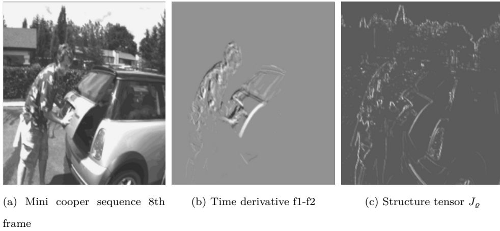
Figure 5.4: Mini cooper image sequence and TV regularization with isotropic case.
