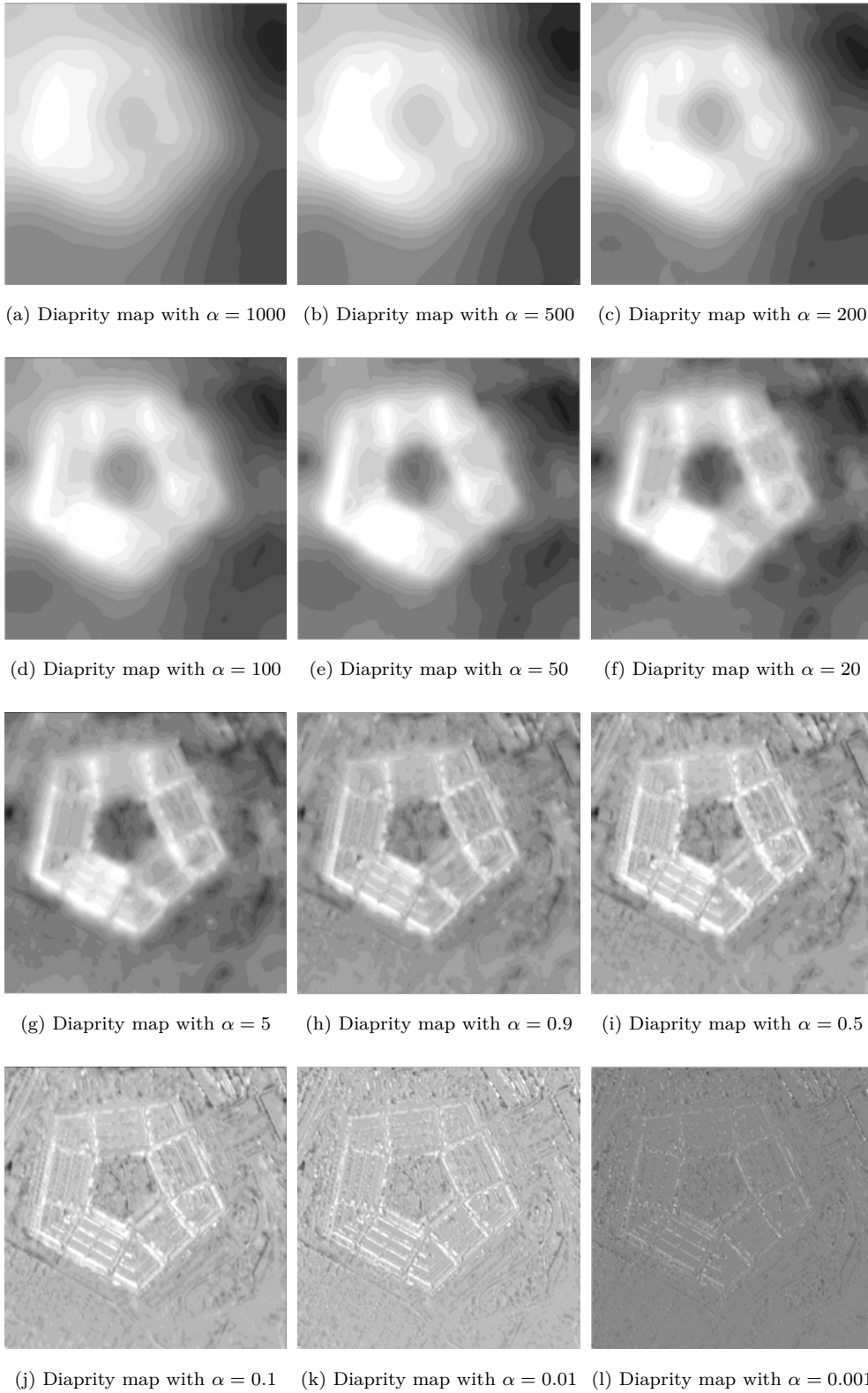
Figure 4.2: Example 1. Disparity map given for various values of \alpha as fixed constant on the whole domain.
