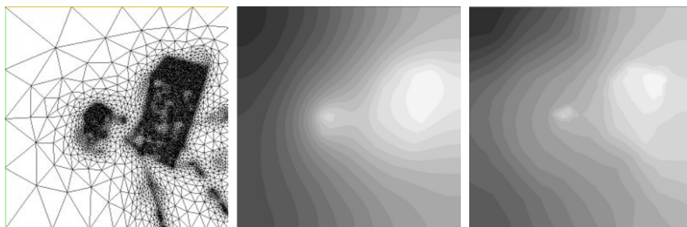
(j) Mesh after iter7
