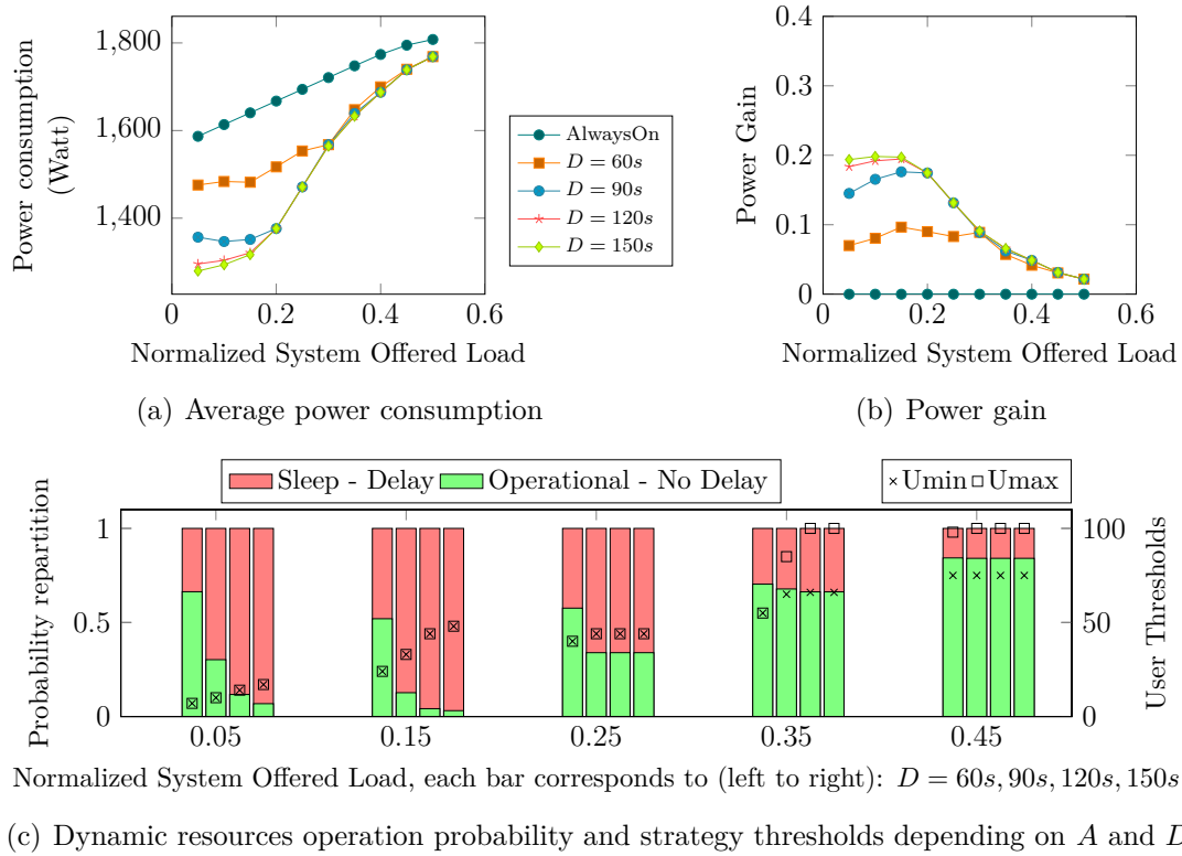
Figure B.1: Results for the Scenario 1, \eta = 1, \gamma_{\max} = 0.05, \delta_{\max} = 0.05 .
