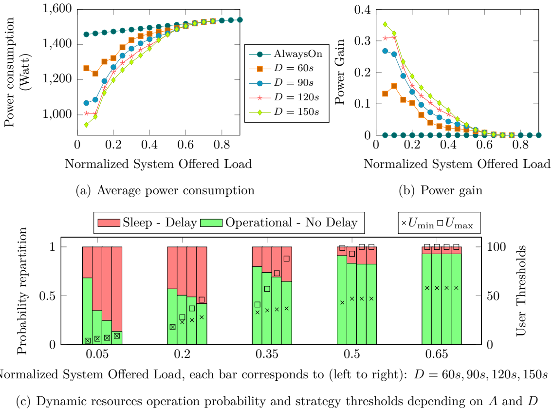
Figure 3.3: Results for the Scenario 4, \eta = 1, \gamma_{max} = 0.05, \delta_{max} = 0.05 .
