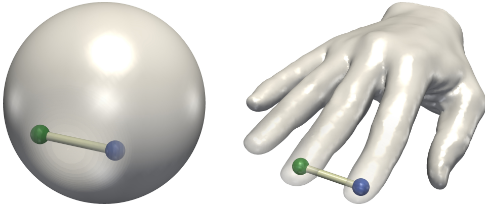
Figure 3.2 – Examples of convex (left) and non-convex (right) 3-manifolds (volumes). On the left, any two points (green and blue spheres) can be linked by a line segment that belongs to the volume (white cylinder). This is not the case for the right volume.
