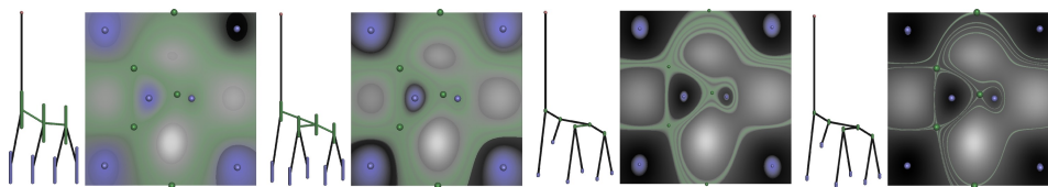
Figure 8.2 – Progressive Join Tree construction illustrated as an uncertain process. The minima and saddles of the finest resolution of the data (gradient of gray in the background) are shown with blue and green spheres respectively. For each data-resolution (from left to right: coarsest to finest) our uncertain topological analysis has been run. The predicted regions for the appearance of minima and saddles are shown in blue and green respectively.
