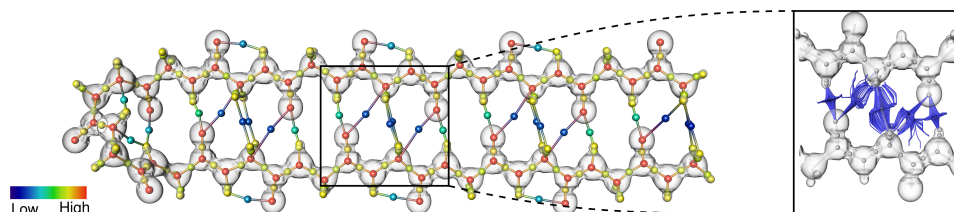
Figure 6.19 – Visual and quantitative exploration of covalent and noncovalent bonds in the \beta -sheet polipeptide. The amplitude of the signed electron density ( |\bar{\rho}| , color-coded from blue to red) enables to distinguish covalent bonds (yellow) from hydrogen bonds (cyan) and van der Waals interactions (dark blue). While the numerical integration of \nabla\bar{\rho} (right inset) enables to visually distinguish the latter two types of interactions, our combinatorial pipeline robustly extracts these features to support further quantitative analysis. In particular, our algorithm reveals the repeating pattern (black frame) of noncovalent interactions responsible for the folding of this molecule, which decomposes it in unitary building blocks corresponding to the elementary amino-acids composing the molecule.
