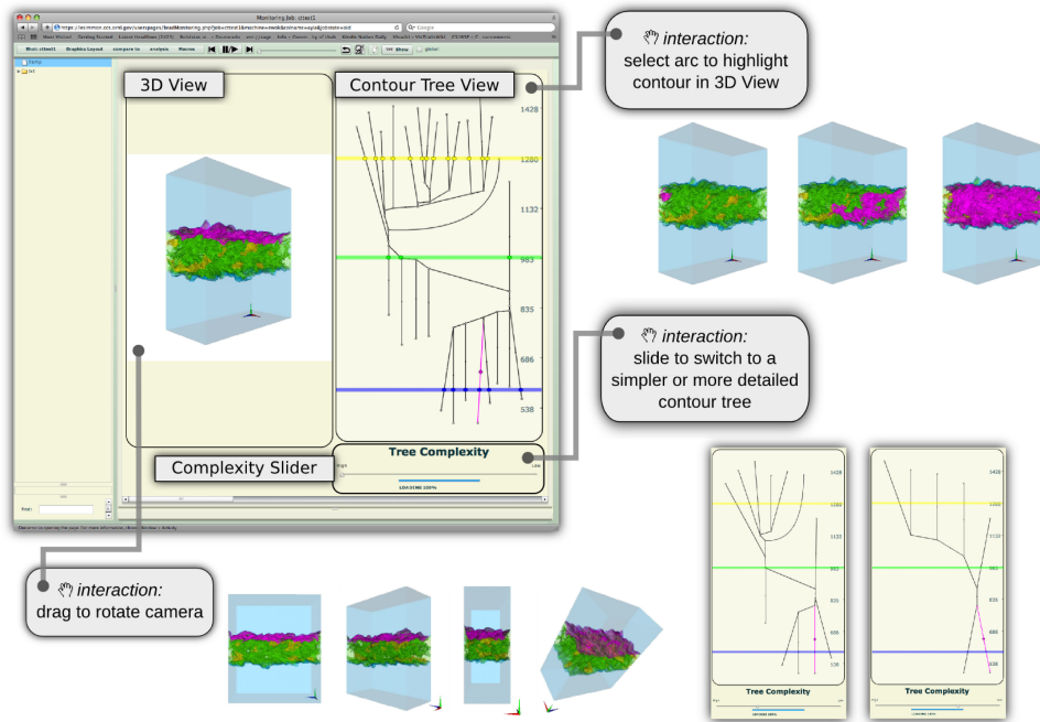
Figure 5.3 – Isosurface based visualization widget for the eSimMon (KVP* 08) web-based simulation monitor: isosurface rendering (top left), Reeb graph planar display (top right), persistence slider (bottom right). Other view examples are provided on the side.
