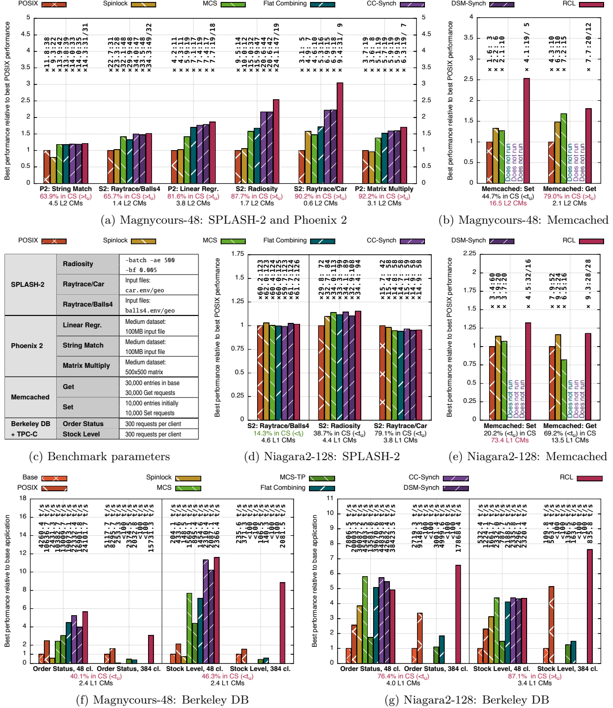
Figure 5.7: Application performance overview
