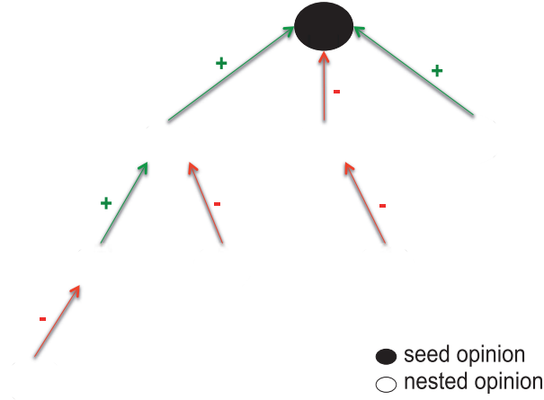
Figure 4.4: Debate Graph
