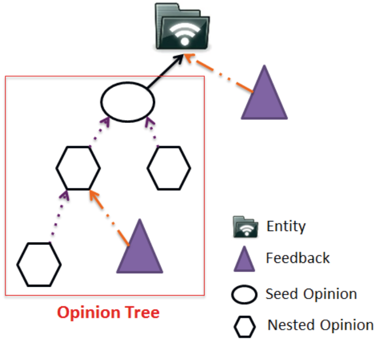
Figure 4.3: Content relations
