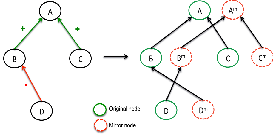
Figure 4.6: Example of a mirror graph
