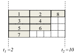
c) Energetic Reasoning with Bin Packing: LB_{ERBPP}=4
