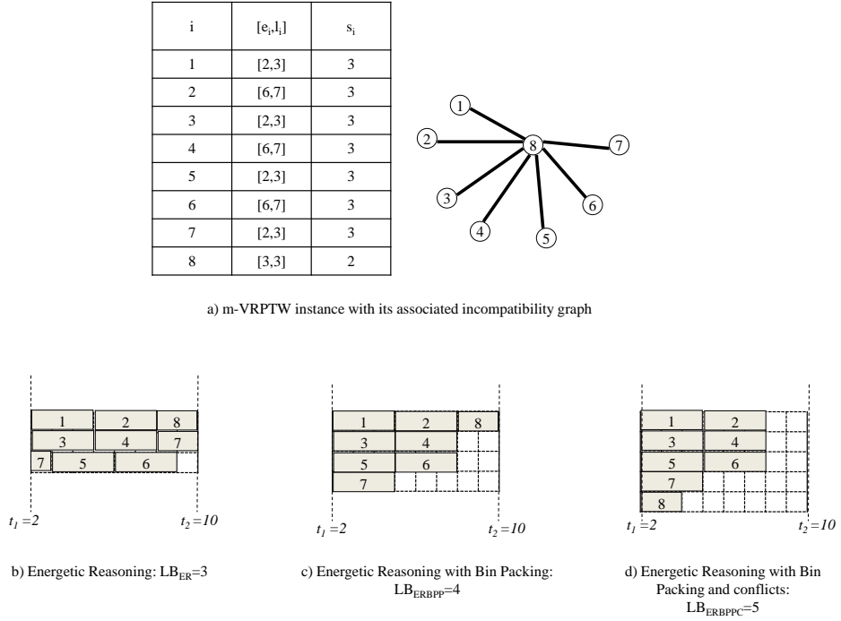
Fig. 2. Illustration of Energetic Reasoning lower bounds.
