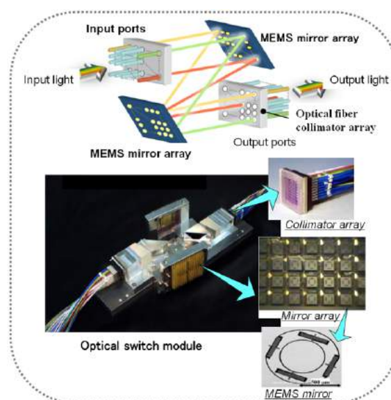
Figure 1.8: The composition of an NxN type optical switch alongside a commercialized product [Boppart, 2013].
