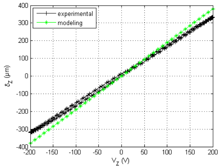
Figure 3.11: Comparison between the experimental values measured along the Z-axis (-+-): 653.7 \mu\text{m} and the afferent modeling (-*-): 760.6 \mu\text{m} .
