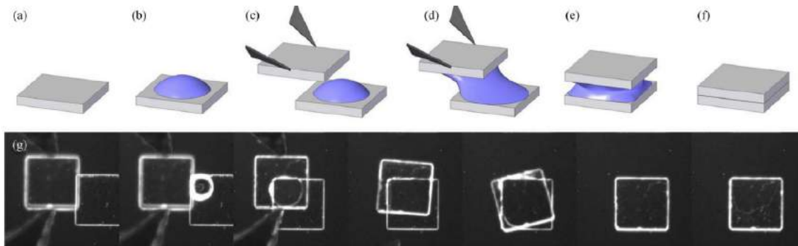
Figure 1.1: Hybrid handling technique [Sariola et al., 2010] of a 50 \times 50 \times 40 \mu\text{m}^3 . (a) Assembly site is on top of a micro-component. (b) Droplet of water is dispensed on the bottom part. (c) Microgripper approaches the release site with a part. (d) Droplet contacts with the top part and wets between the parts, which forms a meniscus. (e) Microgripper releases the part and the capillary force aligns the parts. (f) Water between the two parts evaporates, which leaves the two parts aligned. (g) Image sequence of the actual experiment, as viewed from the top.
