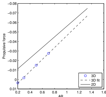
Figure 7.2.2 – Thrust force as a function of the aspect ratio. The solid line represents the force predicted by the 2D approximation and the dashed line is a linear least-squares fit through the available data points from the 3D simulations.
