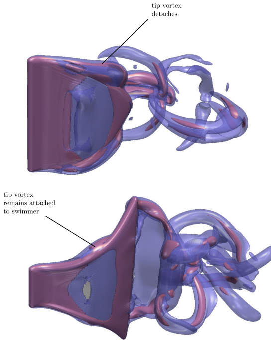
Figure 7.3.3 – Isosurfaces of vorticity magnitude for contacting (top) and expanding shapes (bottom). Blue \|\underline{\omega}\| = 18 , purple: \|\underline{\omega}\| = 9 . In the contracting case, the tip vortices rapidly detach from the swimmer, while they remain close to the surface in the expanding one. This finding may explain the observed difference in performance.
