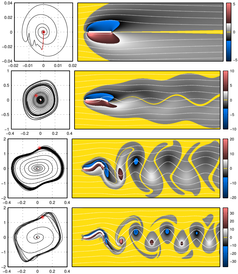
Figure 6.1.2 – The influence of the Reynolds number. Phase-diagram of the trailing edge in the displacement-velocity plane ( y, u_y ) (left column) and a vorticity snapshot (right column) with superimposed white streamlines. Only part of the computational domain is shown. The Reynolds number is Re = 25, 100, 200, 1000 (from top to bottom). The point in phase space belonging to the snapshot is marked with a red star.
