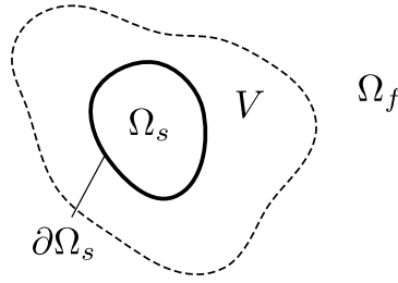
Figure 2.4.1 – Computation of hydrodynamic force.
