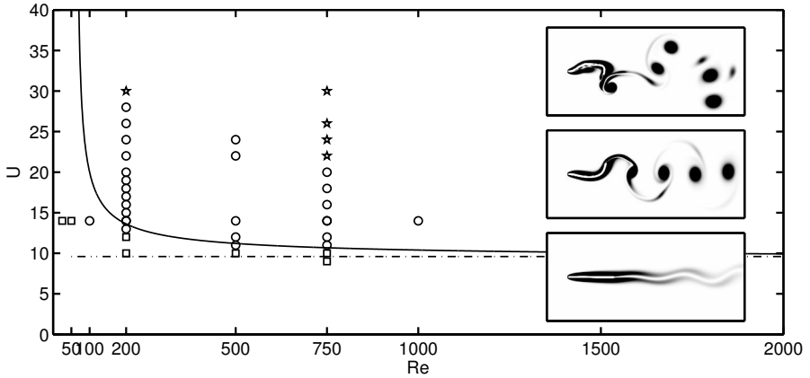
Figure 6.1.1 – Stability map in the Re-u^* plane for \mu = 1/3 . Inviscid [109] (–·) and viscous linear stability analysis [25] (–). Symbols indicate present simulations, found to be stable ( \square ) or in an either periodic ( \circ ) or chaotic ( \star ) fluttering state. Insets show corresponding snapshots of the absolute vorticity |\omega| at Re = 750 .
