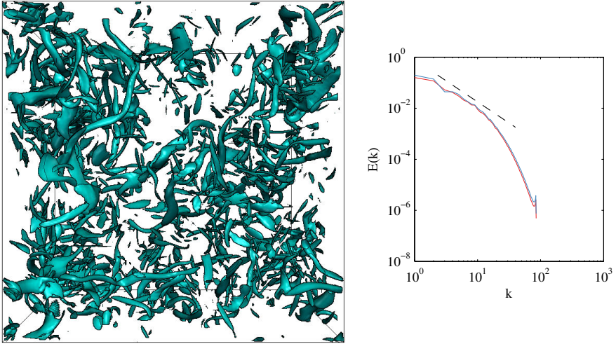
Figure 4.3.2 – Homogeneous isotropic turbulence. Left: visualization of the flow field by the \|\underline{\omega}\| = 18 isosurface of absolute vorticity. In the simulation R_\lambda is equal to 100, and the typical “vortex tubes” [79] are visible. Forcing method is negative viscosity (Jiménez). Right: energy spectrum for both forcing types, dashed line is k^{-5/3} .
