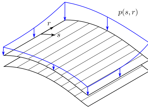
Figure 5.2.2 – Surfaces forces on the beam in a 3D configuration, where it becomes a plate with one rigid direction ( r ). The pressure is interpolated on the top- and bottom surfaces, and the resulting force is normal to the surface.
