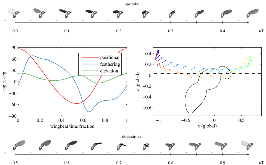
Figure 3.1.3 – Fruit fly in hovering with the kinematics data according to [57]. Top and bottom row show the wingbeat during up- and downstroke. Centered figures illustrate the wing angles (left) and the wing trajectory (right). Dashed line is the stroke plane.
