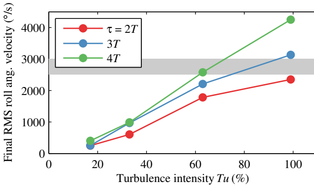
Figure 4.3.7 – RMS value of the final roll angular velocity \Omega_{roll} versus the inflow turbulence intensity, calculated over all flow realizations. Different colors correspond to different response delay times \tau . The gray shaded area represents the limit of sensor saturation [138, 170], see text for details.
