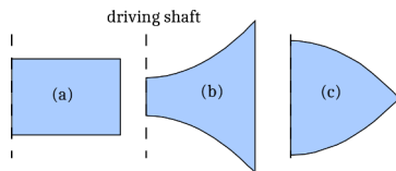
Figure 7.3.1 – Different shapes investigated here, termed (a) “rectangular”, (b) “expanding” and (c) “contracting”. All three shapes have the same surface.
