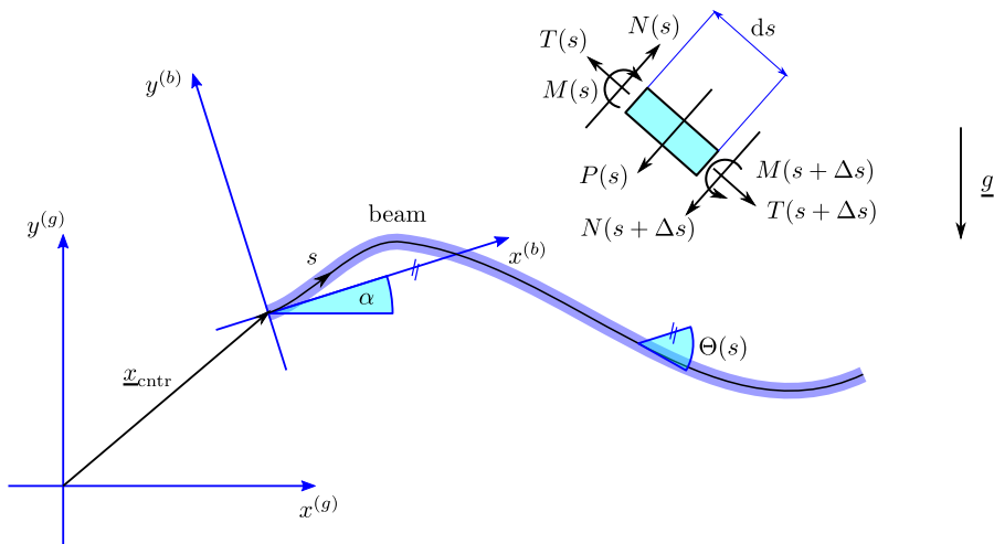
Figure 5.1.2 – Derivation of the beam equation. The slender, inextensible beam is clamped in the relative reference frame x^{(b)}, y^{(b)} , which is translated by \underline{x}_{\text{cntr}} and rotated by \alpha with respect to the global reference frame. The governing equations are derived considering the beam element (inset) with the forces and moments acting on it. Gravity is assumed in negative y^{(g)} direction.
