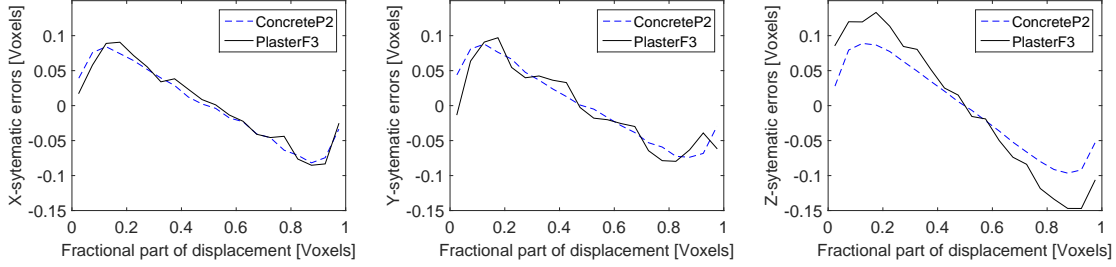
Figure 8.1: Comparison of DVC systematic errors for EPS concrete and EPS plaster specimen
