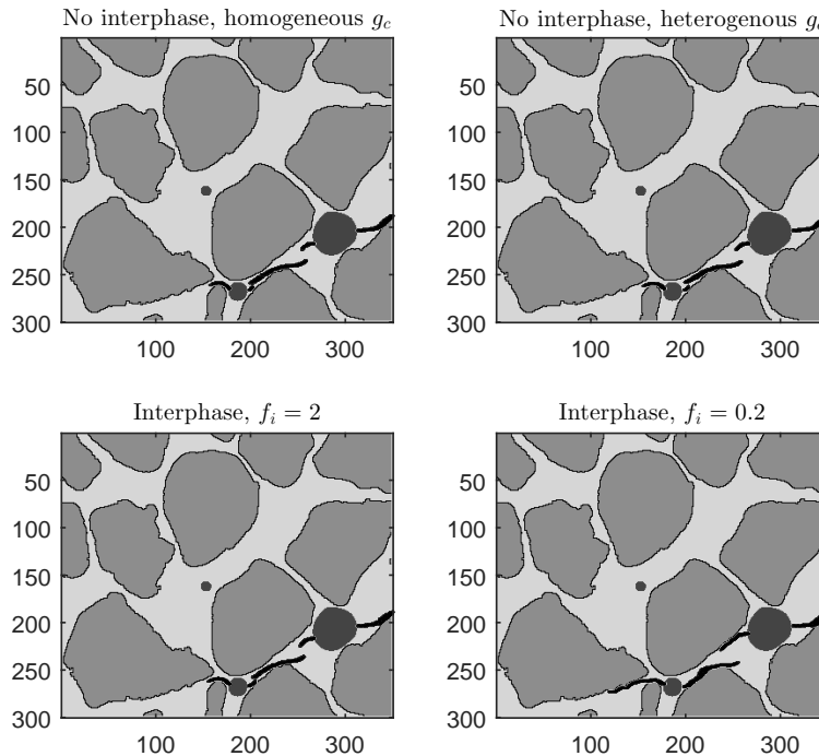
Figure 3.4: Comparison of cracks networks obtained by 4 models. The cracks are depicted in black.
