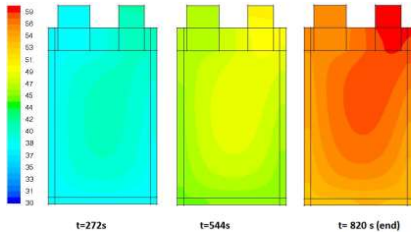
Figure 3.22: Thermal distributions based on modeling at 4I_t discharge current rate at 20^{\circ}\text{C} of environment temperature
