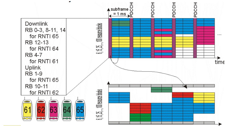
Figure 2.4: LTE control and data region, source [4]
