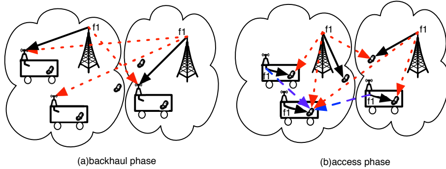
Figure 5.6: Interference illustration in FDD mobile relay mode with frequency reuse (the useful signal is represented in solid line, interference is represented in dashed line)
