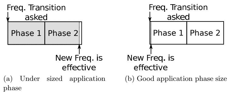
Figure 8.17: Frequency transition latency versus phase duration
