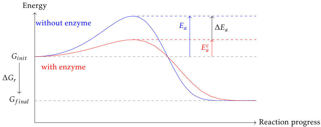
Figure 2.1: Energy of the system as a function of the state of a single molecular reaction event. The reaction releases per mole an energy |\Delta G_r| and each microscopic conversion requires an activation energy E_a to take place, this activation energy is reduced to E_a^c when it is catalysed by an enzyme.
