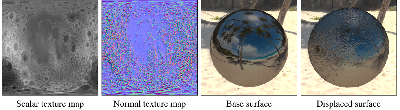
Figure 3.2 – Overview of the displacement mapping technique. Displacement mapping consists in displacing a surface along its geometric normal using a scalar texture map, and using a normal texture map to compute the final shading. Here, the scalar texture map is visualized as grey-scale values, while the normal texture map is color-coded.
