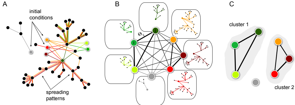
Figure 6.17: Schematic representation of the cluster detection procedure. (A) Different simulated invasion paths (colored lines) obtained for different seeder (colored nodes) are shown on the network. Each path is colored according to with the color of the seeding node. (B) The initial conditions similarity network (ICSN) is obtained by calculating the overlap \Theta_{ij} for any pair of initial conditions i and j , measuring the similarity between the invasion paths originated by the two nodes. Thicker lines in the ICSN indicate a higher overlap. (C) By filtering the ICSN neglecting all links characterized by an overlap lower than a given threshold \Theta_{th} , two non-trivial connected components emerge (i.e. with a size larger than one farm) corresponding to cluster 1 and cluster 2 of nodes leading to similar propagation pathways.
