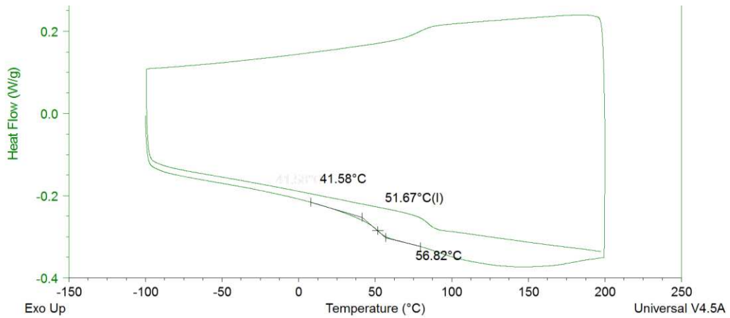
Appendix 9: Glass transition measurement for Infused material at saturation time.
