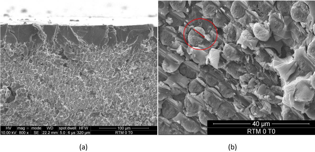
Figure 67: SEM observation on tensile fracture surface on UD RTM laminates loaded in the fibre direction, before ageing. Region on specimen surface (a), focus on fibres (b).
