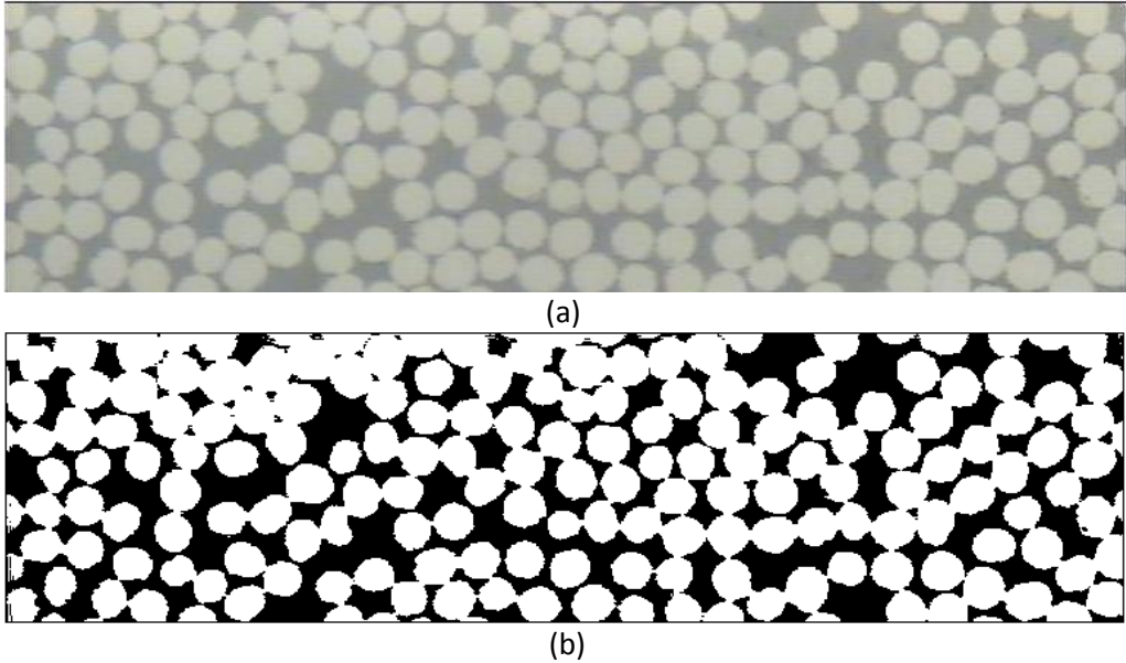
Figure 60: Example of optical microscope observation (a) and ImageJ treatment (b) for UD 2.5 mm RTM material (perpendicular to fibres, fibre diameter is approximately 5µm).
