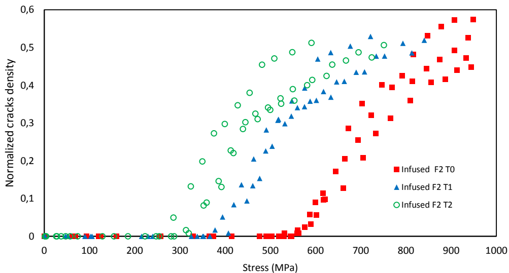
Figure 109: Evolution of normalized crack density for infused composite [0 2 ,90 2 ] s before ageing (red square), at saturation (blue triangle) and at saturation time plus one month (green circle) (3 specimens per condition).
