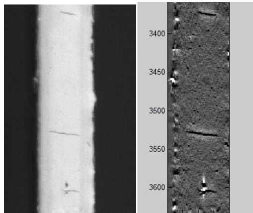
Figure 38 : Visualization of cracks before (left) and after (right) Matlab™ processing on a [0,90]_{2s} sample.
