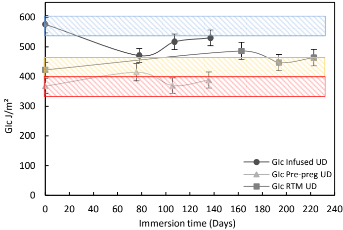
Figure 112: Evolution of critical strain energy release rate G_{ic} in carbon/epoxy Pre-preg, Infused and RTM materials during sea water ageing.
