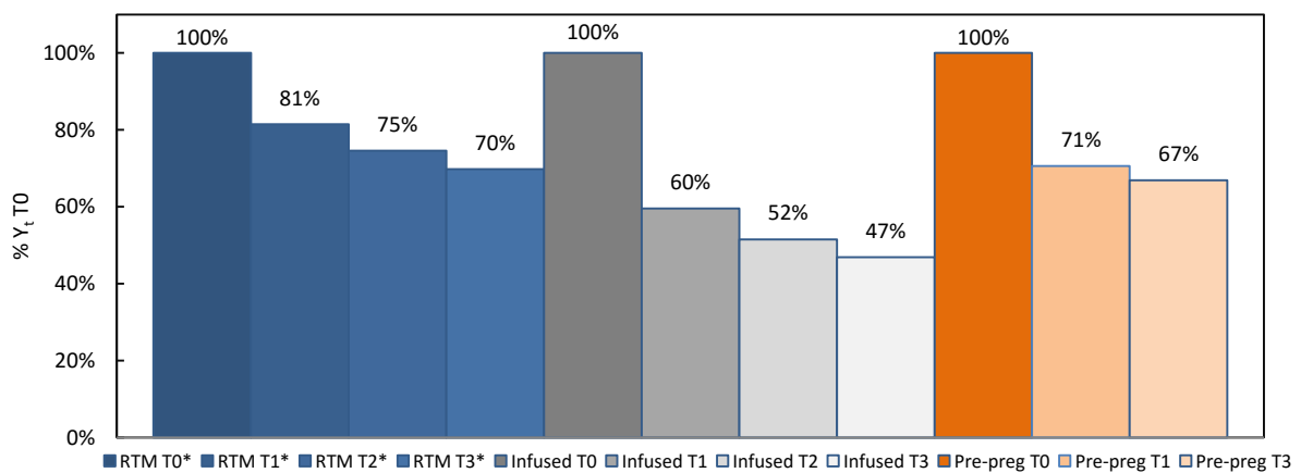
Figure 144: Evolution of normalized longitudinal tensile strength X_l , during sea water ageing for the three materials.
