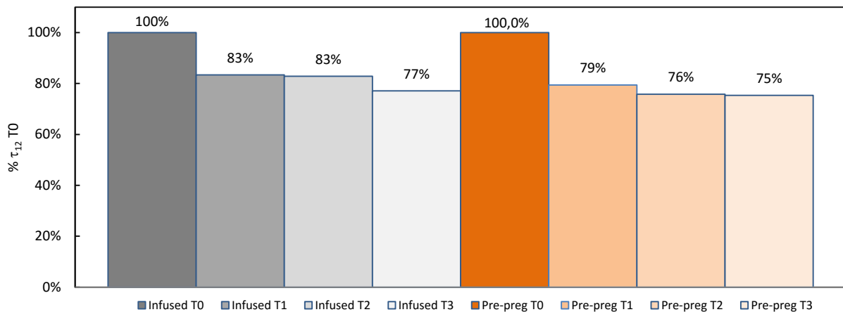
Figure 146: Evolution of normalised in-plane shear strength \tau_{12} , during sea water ageing for Infused and Pre-prep materials.
