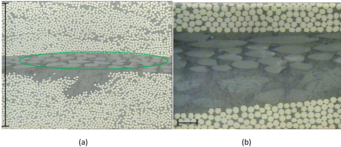
Figure 58: Microscope optical observation of RTM UD (average scales: (a) 0.38mm (b) 20μm).
