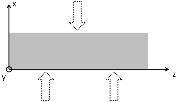
Figure 53: Out-of-plane compression mechanism in unidirectional composite. Shear ILSS test leads to \tau_{13} if 0° plies are oriented in (y,z) plan or leads to \tau_{23} if 90° are oriented in (y,z) plan.
