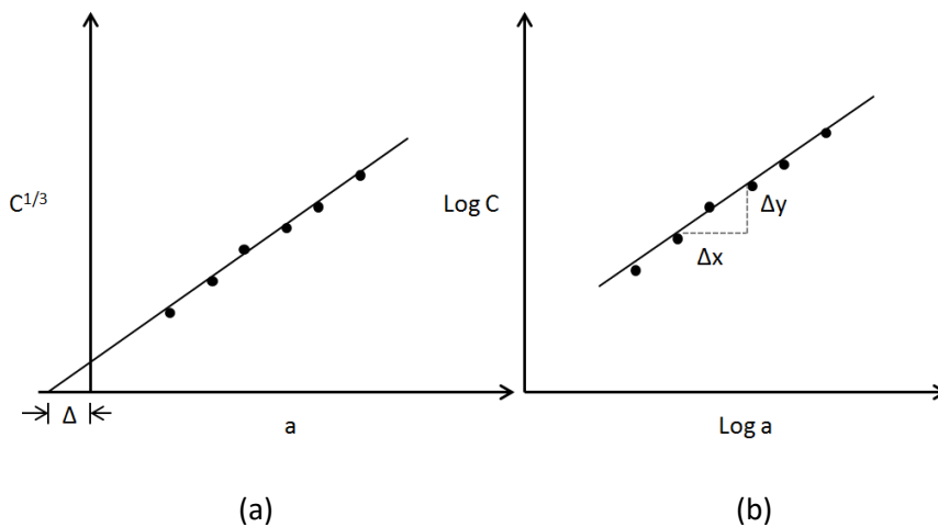
Figure 47 : Modified Beam Theory (a) and Compliance calibration (b) for DCB test.
