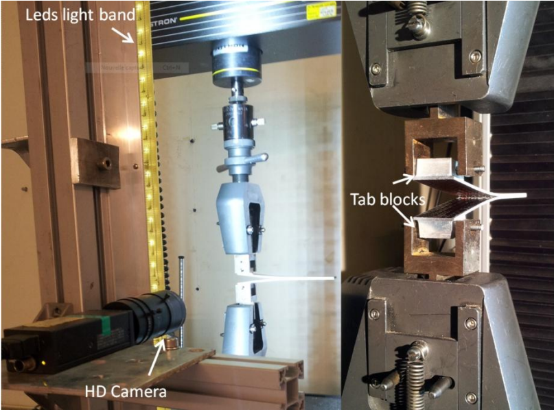
Figure 45: DCB test set-up.
