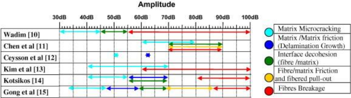
Figure 36 : Amplitude distribution according to the damage mechanisms in composite materials [126].
