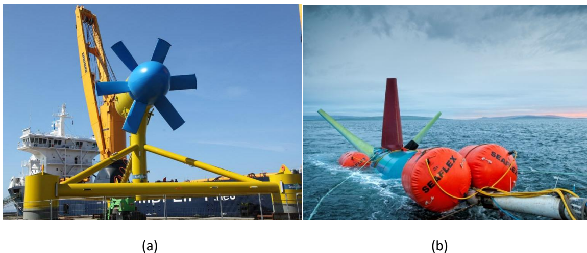
Figure 2: Sabella D10 Tidal turbine (a) and CoRMAT tidal turbine with 4 m RTM blades, courtesy of Airborne Marine and Nautricity Ltd (b).
