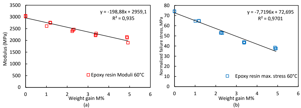
Appendix 14: Evolution of pure resin tensile modulus (a) and strength (b) versus water content, aged at 60°C.
