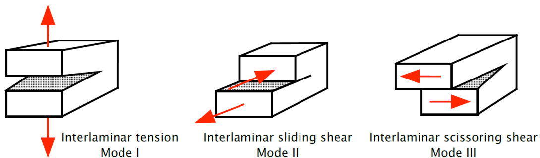
Figure 42 : Fracture test loading modes
