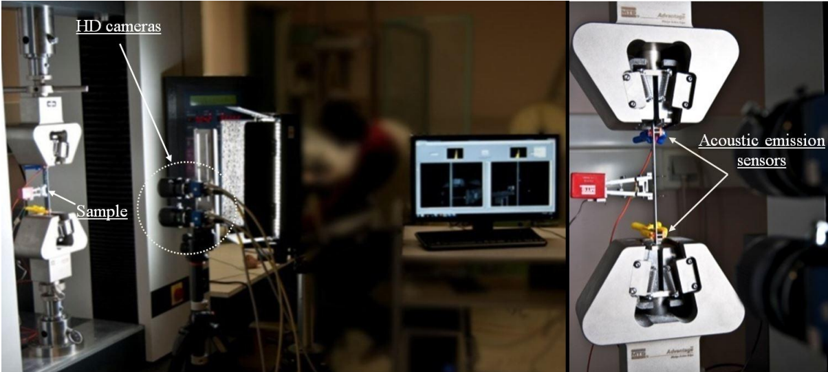
Figure 37 : Test set-up to measure intralaminar tensile cracking.
