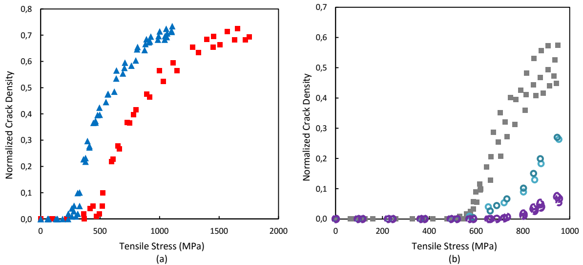
Figure 41: Evolution of normalized crack density as a function of applied stress for Pre-preg (a) and Infused (b) materials. Pre-preg [0_2,90_2]_s : blue triangles, Pre-preg [0_2,90_{1/2}]_s : red squares, Infused [0_2,90_2]_s : grey squares, Infused [0,90,0,90]_s : blue circles for centre 90_2 and purple circles for single 90^\circ plies on specimen sides.
