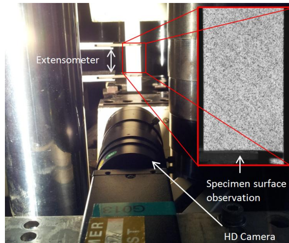
Figure 27: Test procedure for the determination of in plane shear response of composites.
