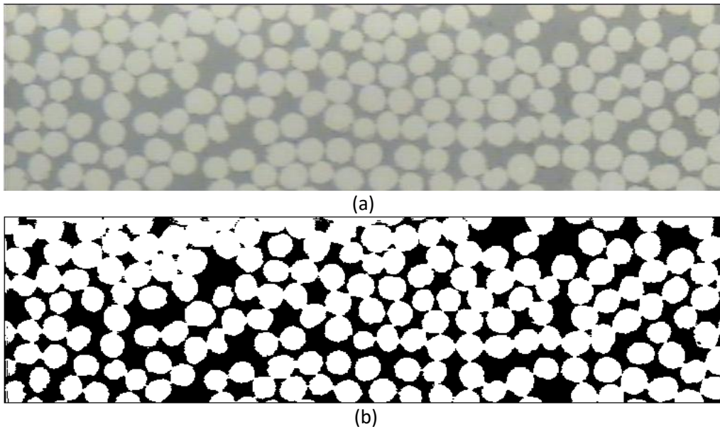
Figure 60: Example of optical microscope observation (a) and ImageJ treatment (b) for UD 2.5 mm RTM material (perpendicular to fibres, fibre diameter is approximately 5 \mu m).
