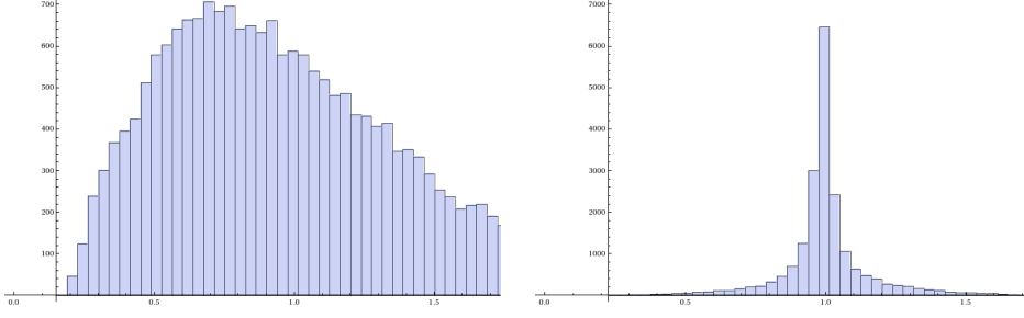
Figure 8.4: Distribution of masses for points on the Calabi-Yau quintic Z_0^5 + Z_1^5 + Z_2^5 + Z_3^5 + Z_4^5 - 0.246 \times Z_0 Z_1 Z_2 Z_3 Z_4 , using 1 Fubini-Study metric (left) and 19 Fubini-Study metrics & subsets, optimally chosen (right).
