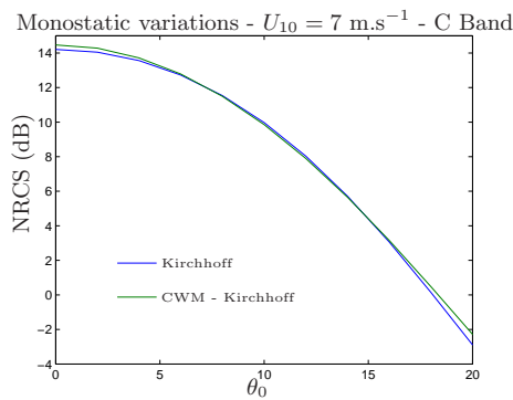
Figure 6. Monostatic variation of the NRCS. Upwind-wind configuration in C-Band for a 7 \text{ m.s}^{-1} wind speed.
