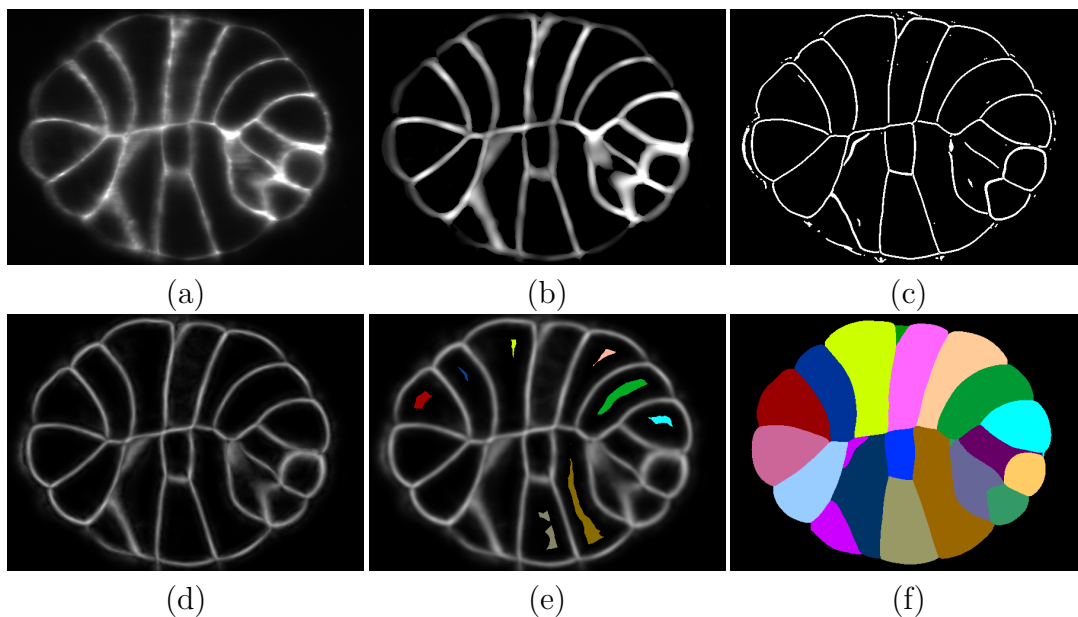
Figure 3.6 – Cell segmentation framework. (a) A section through a 3D embryo image. (b) Planar response filter. (c) Thresholded extrema. (d) Surfacedness map after tensor voting. (e) Seeds detection. (f) Cell segmentation by seeded watershed.
