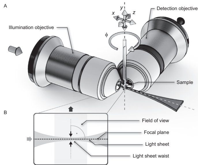
Figure 1.8 – Principle of light-sheet microscopy. The light-sheet goes through the illumination objective. The detection objective is perpendicular to the illumination objective and allows to image the whole field of view created by the light-sheet. (adapted from [Weber et al., 2014])
