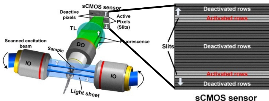
Figure 1.10 – Principle of slit mode in scanned light-sheet microscopy. The lasers, seen here coming from both sides of the embryo, are focused by corresponding illumination objectives (IO). The emitted photons then go through the detection objective (DO) to be captured by the sCMOS camera where only the rows that are meant to receive light are activated. Adapted from [Yang et al., 2015]
