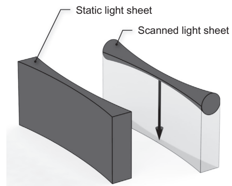
Figure 1.9 – DSLM [Weber et al., 2014]
