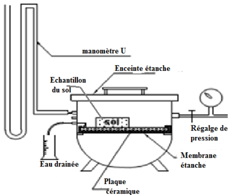
Figure II-4: Cellule de Richards
