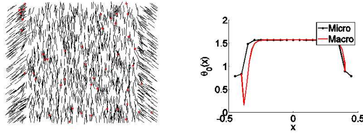
Figure 3.8: (A) Simulations of the microscopic model with \varepsilon = 0.1 , external potential c_u = 0.01 and fiber linking/unlinking frequencies such that \chi = 0.1 (first line). From A1 to A3: for increasing values of the microscopic noise d : d = 10^{-5} , d = 10^{-4} and d = 10^{-3} . For each, we show the profiles of the solutions averaged over the y direction and over 10 simulations for the microscopic model (black curves, second line). For each set of parameters, we superimpose the profiles of the solutions to the macroscopic model (red curve). For small d and small external potential c_u = 0.01 (A1,A2), fiber orientation angles reach \frac{\pi}{2} and -\frac{\pi}{2} on the left and right hand sides of the domain, with a zone of quasi horizontal fibers in the middle, as predicted by the macroscopic model. For increasing d (A3), the profile flattens and fibers no longer reach the orientation angles \frac{\pi}{2} . The macroscopic model captures the same features for the same parameters. (B) Case c_u = 0.1 . In this case, all fibers reach orientation \pm\frac{\pi}{2} due to the large intensity of the external potential for both the microscopic and macroscopic model.
