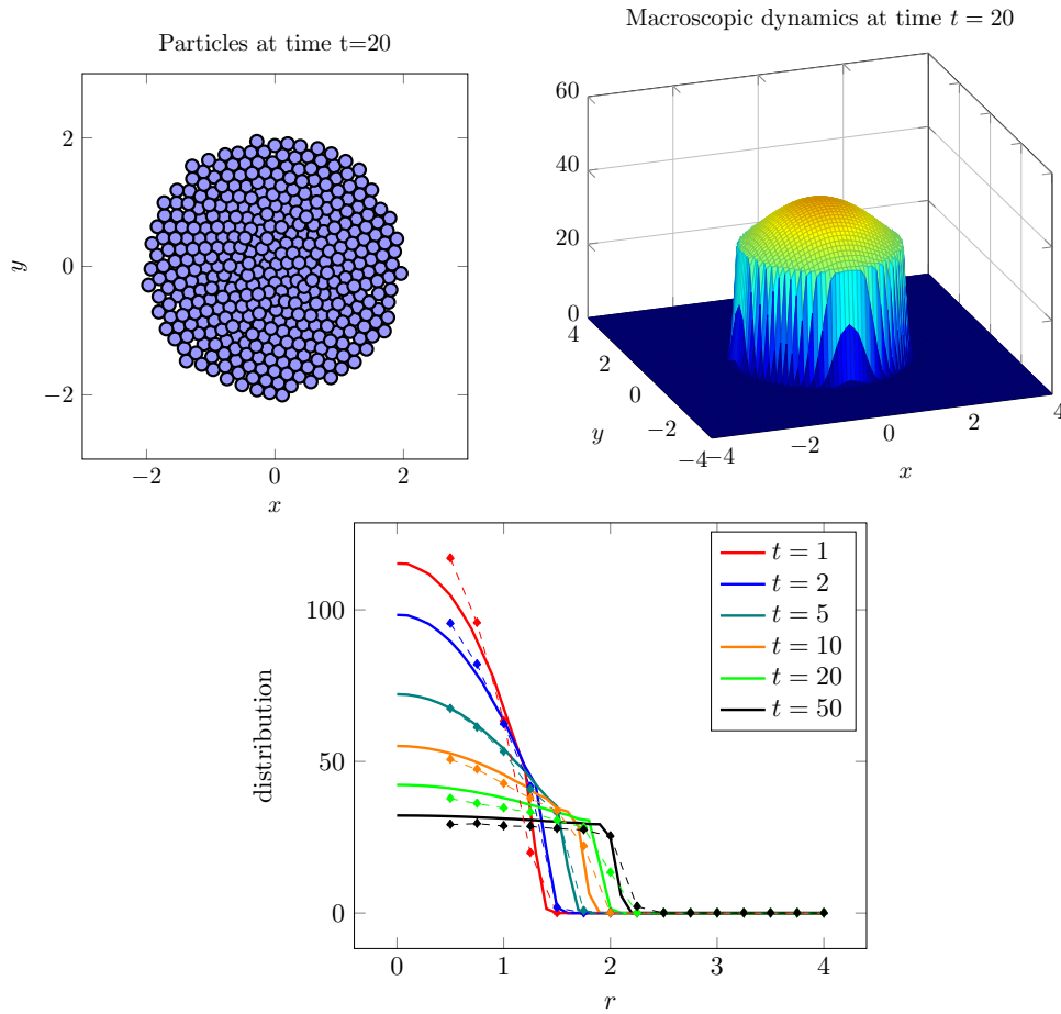
Figure 4.24: Top-left : positions of the particles after t = 20 unit time running the microscopic dynamics (2.1). Parameters: N = 400 particles, R = .1 , \alpha = -1 , \Delta t = 10^{-1} . Top-right : density \rho(x, t) solution of the macroscopic dynamics (3.1). Bottom : radial distributions for the micro- and macro- dynamics (resp. diamond and plain).
