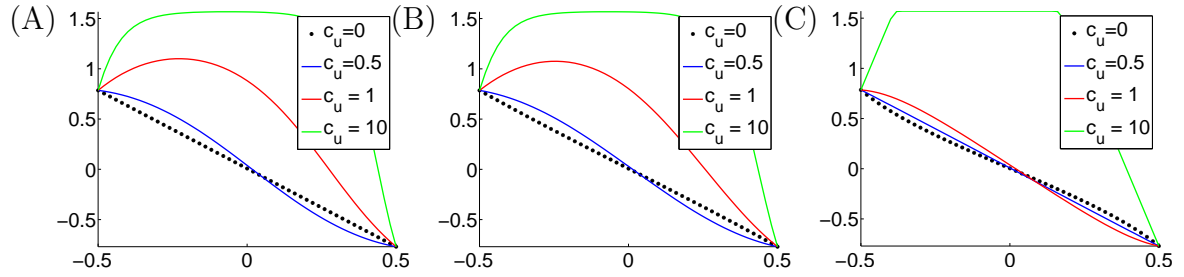
Figure 3.5: Profiles of the solutions to (3.43)-(3.41) for \alpha_2 = 0.1 , \theta_1 = \frac{\pi}{4} , \theta_2 = -0.98\frac{\pi}{4} (assymmetric boundary conditions). Black dots: c_u = 0 , red curve: c_u = 1 , green curve: c_u = 10 . (A) \alpha_3 = 0 , (B) \alpha_3 = -0.05 , (C) \alpha_3 = -0.1 .
