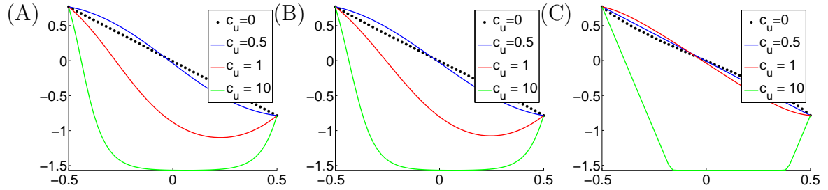
Figure 3.4: Profiles of the solutions to (3.43)-(3.41) for \alpha_2 = 0.1 , \theta_1 = 0.98\frac{\pi}{4} , \theta_2 = -\frac{\pi}{4} (assymmetric boundary conditions). Black dots: c_u = 0 , red curve: c_u = 1 , green curve: c_u = 10 . (A) \alpha_3 = 0 , (B) \alpha_3 = -0.05 , (C) \alpha_3 = -0.1 .
