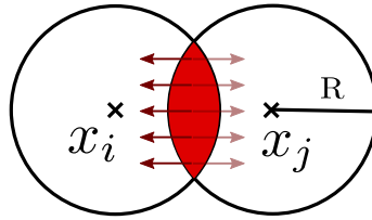
Figure 4.17: The two particles located at x_i and x_j interact when they are at a distance less than 2R from each other. On this region, the modified empirical distribution \tilde{\rho} is larger than the threshold \rho_* = \frac{1}{\pi R^2} .
