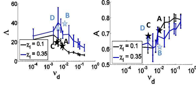
Figure 1.18: Statistical Quantifiers \Lambda and A of the simulations of Main Text (see Fig. 3 (I) of Main Text), with random insemination, flexural modulus c_1 = 1 , as functions of the fiber unlinking frequency \nu_d for two different linked fiber fraction \chi_\ell = 0.1 (black curve) and \chi_\ell = 0.35 (blue curve). The mean fiber cluster elongation \Lambda is a non monotonous function of the unlinking frequency \nu_d , that first increases and then decreases with \nu_d \in [10^{-3}, 0.1] . The mean alignment of the fiber clusters A increases with \nu_d , with two plateau values for \nu_d \leq 10^{-3} and \nu_d \geq 10^{-1} . Values corresponding to the simulations of Main Text with biased insemination with biasing parameter \alpha = 10^{-3} are indicated as blue stars for \chi_\ell = 0.35 and black ones for \chi_\ell = 0.1 . The values of A and \Lambda for random and biased inseminations are similar in the range of \nu_d \in [10^{-3}, 10^{-2}] .
