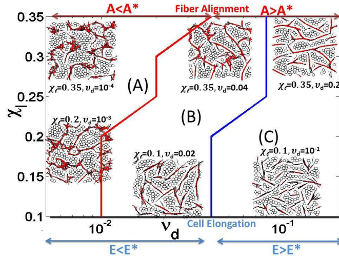
Figure 1.19: Phase diagram representing the separation lines between the three morphologies (A), (B) and (C) (Phase (A): A < A^* and E < E^* ; Phase (B): A > A^* and E < E^* ; Phase (C): A > A^* and E > E^* ), as function of the unlinking frequency \nu_d and of the linked fiber fraction \chi_\ell . The separatrix A = A^* between Phases (A) and (B) is plotted in red, while the separatrix E = E^* between Phases (B) and (C) is plotted in blue. For each phase, two simulations in the corresponding range of parameters \nu_d and \chi_\ell are shown.
