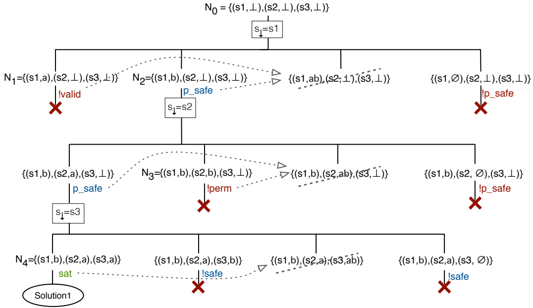
Figure 5.8: Search tree for our example. The choice of states s_{\downarrow} , which define the tree structure, are mentioned in frames. The nodes that are crossed out or unmentioned are not generated and checked. The dotted lines corresponds to the pruning of combined siblings. The results of the tree traversal is the only node labelled by sat .
