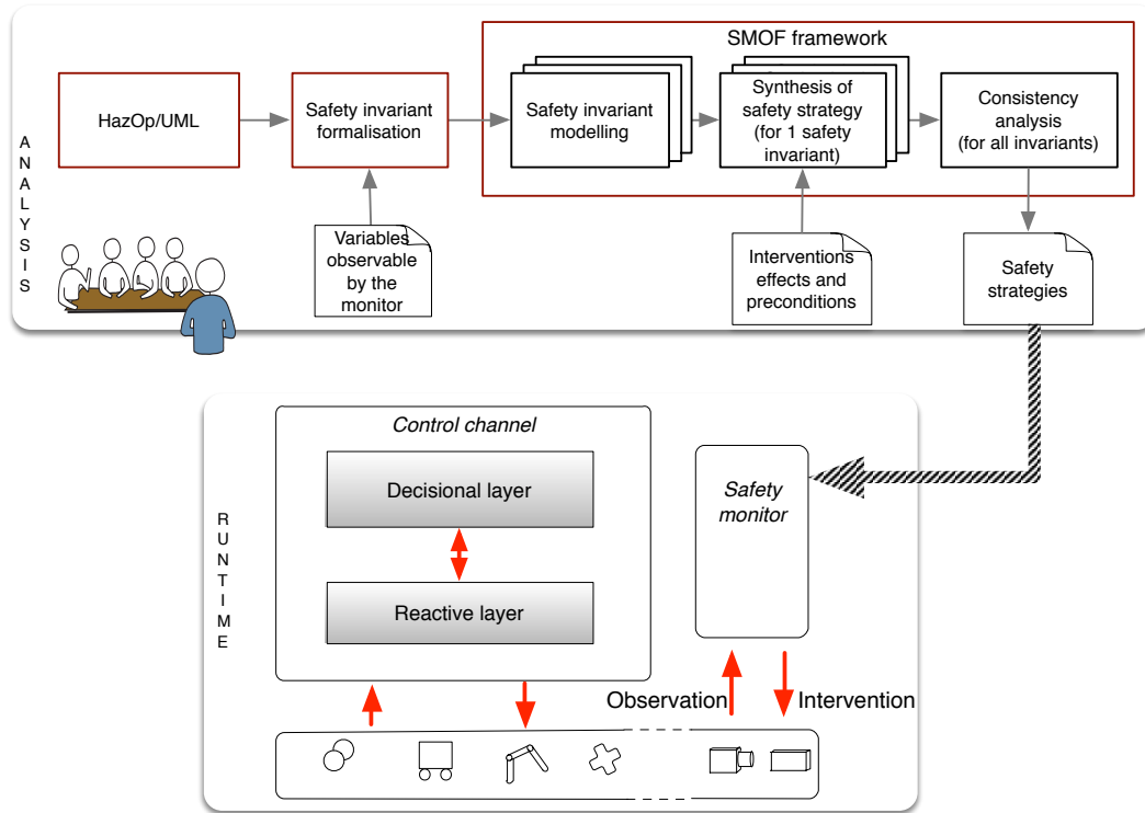
Figure 5.2: Overview of the process
