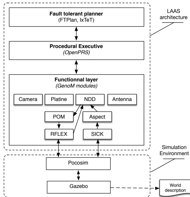
Figure 4.6: Simulation environment
