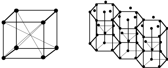
Figure 2: 3D-appearance models
