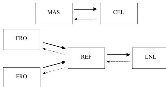
Figure 16 : substitutions
