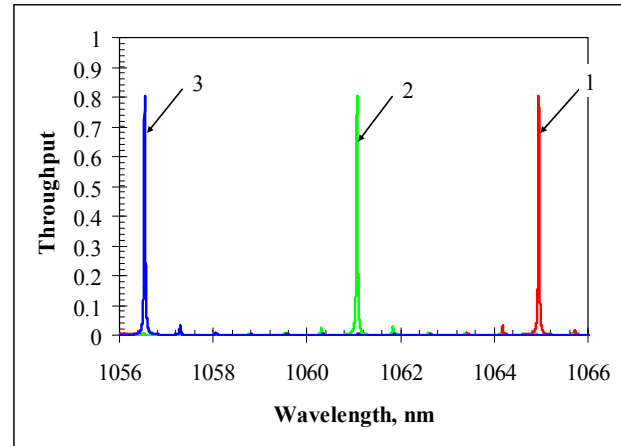
Fig. 4.2-7. Throughput of the FPB filter for 1064 nm region, for different inclination ( \alpha ) of the reflecting VB: curve 1: \alpha \sim 2.8^\circ , curve 2: \alpha \sim 7.9^\circ , curve 3: \alpha \sim 11.2^\circ )
