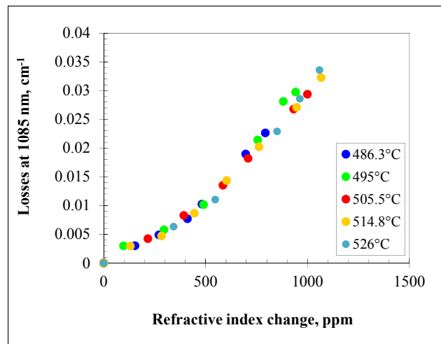
Fig. 3.2-13. Dependence of the losses on refractive index change after thermal development at different temperatures from 485 to 525^\circ\text{C} and for different durations.
