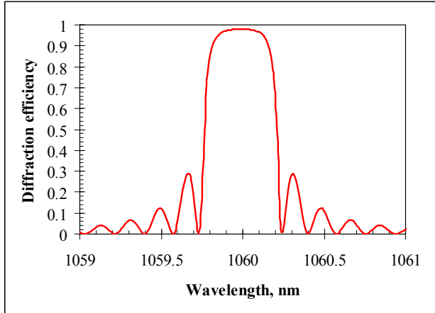
Fig. 4.2-1. Typical spectral dependence of the diffraction efficiency on incident wavelength of a RBG.
