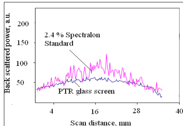
Fig. 4.4-2. Evolution of the back scattering across the aperture of a 2.4 % Spectralon standard and PTR glass holographic screen.
