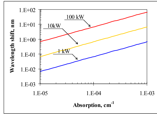
Fig. 3.2-7. Bragg wavelength shift in a conventionally cooled in air PTR glass plate versus the absorption coefficient for different incident power of laser beams.
