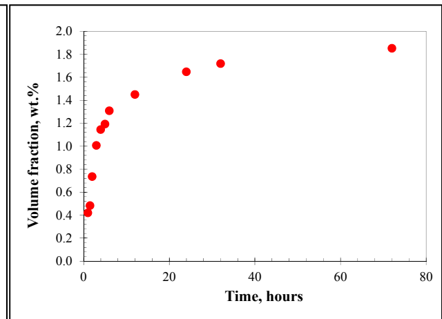
Fig. 3.2-11. Dependence of volume fraction of NaF crystals in PTR glass on duration of thermal development at 515°C.
