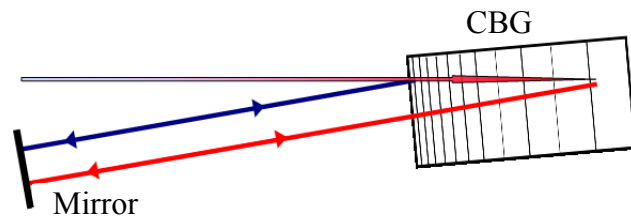
Fig. 4.6-2. A tilted CBG with an external retroreflecting mirror which provides double pass of a laser pulse.
