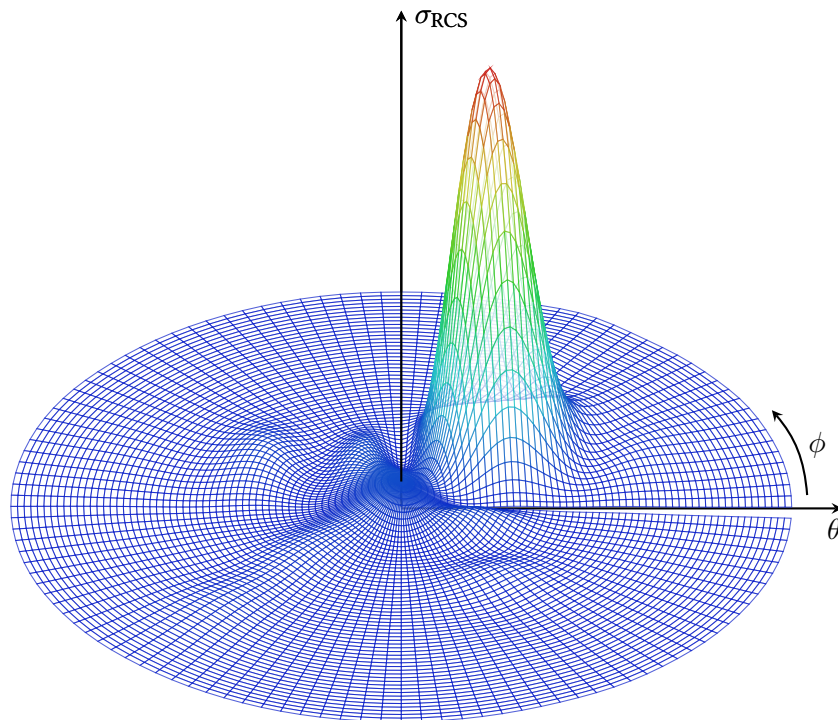
Figure 8.17 | Radar cross-section of an ideal 2D dielectric reflectarray at frequency f . \theta varies from 0 to 90°, while \phi varies from 0 to 360°. The directivity peak is observed around (\theta, \phi) = (28.5^\circ, 45^\circ) , with an efficiency close to 60%. Several parasitic lobes are observed, particularly around the normal direction (\theta, \phi) = (0^\circ, 0^\circ) .
