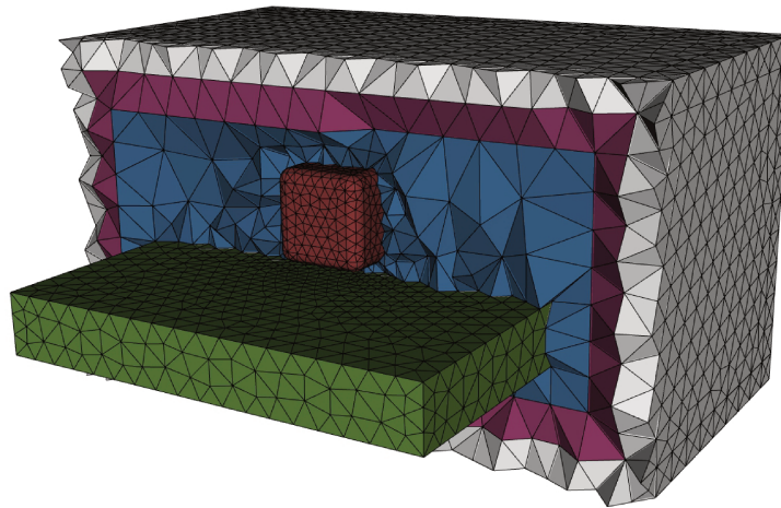
Figure 5.15 | Nanocube mesh with rounded corners. The silver cube (in red) is put on a gold layer (in green), both enclosed by the total field region (in blue). The latter is surrounded by a TF/SF interface on which the incident field is imposed. Then, we find the scattered field region (in purple), surrounded by PMLs (in gray).
