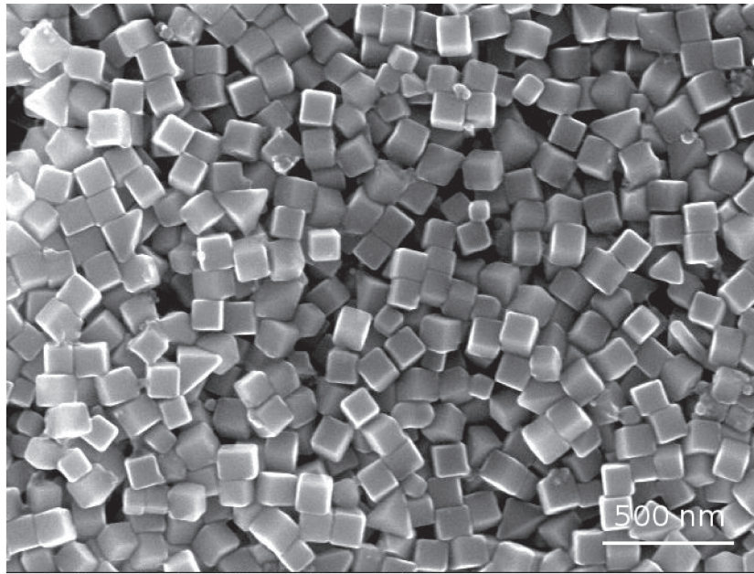
Figure 8.4 | Random arrangement of chemically-produced nanocubes. Courtesy of A. Moreau.
