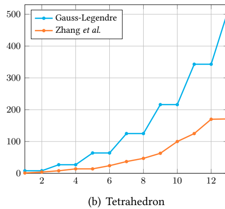
Figure 5.6 | Number of integrations points required by Gauss-Legendre and [ZCLO9] rules on triangle and tetrahedron.
