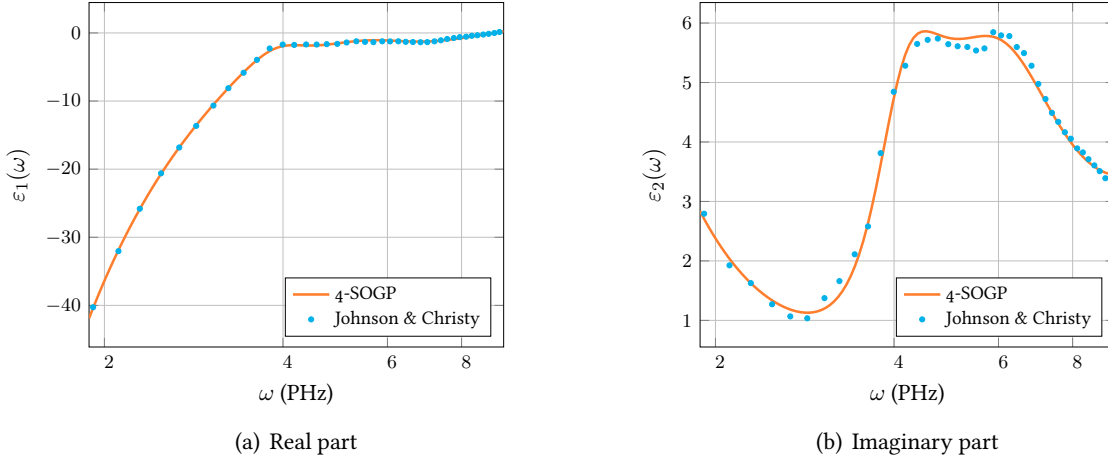
Figure 2.6 | Real and imaginary parts of the gold relative permittivity predicted by the 4SOGP model compared to experimental data from Johnson & Christy. The parameter values can be found in appendix A.
