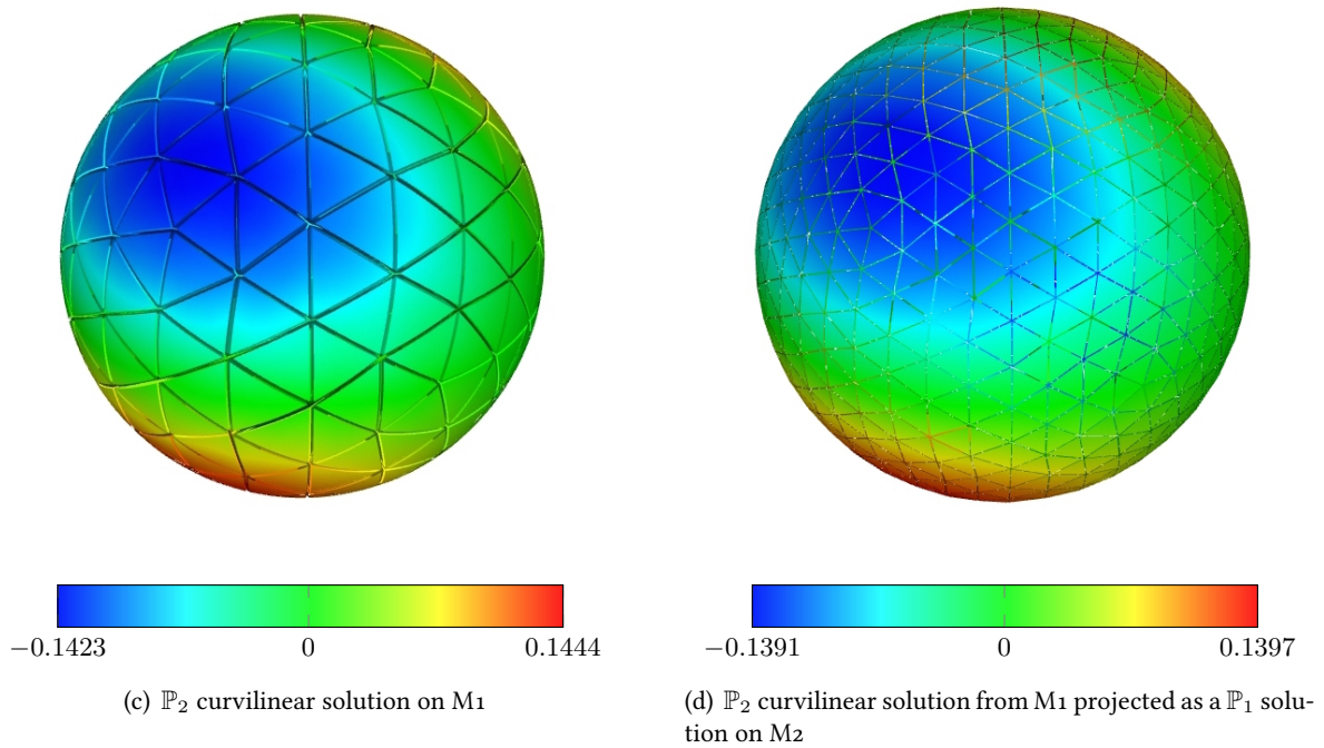
Figure 5.10 | \mathbb{P}_2 curvilinear numerical solution of the spherical cavity mode on the M_1 mesh projected as a \mathbb{P}_1 solution on the M_2 mesh.
