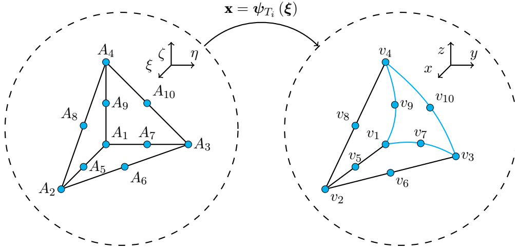
Figure 5.3 | Second order mapping from the reference element \hat{T} to the physical element T_i .
