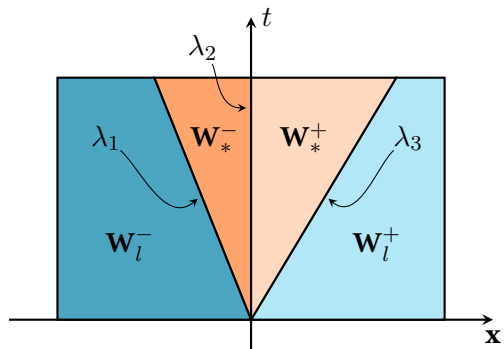
(d) Solution of the leading term Riemann problem
