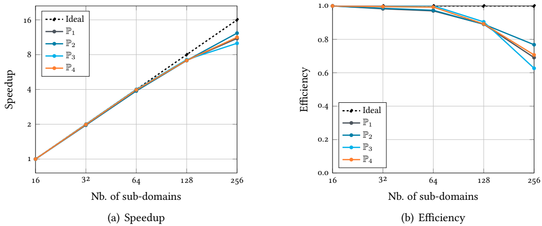
Figure 7.7 | MPI speedup and efficiency for the PEC cavity case on mesh M1, for 16 to 256 subdomains.
