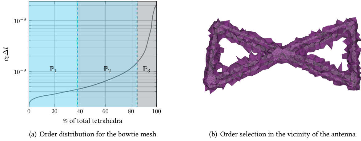
Figure 6.13 | Polynomial order repartition for the bowtie mesh with respect to timestep (left), and geometrical repartition (right) for the \mathbb{P}_1 - \mathbb{P}_3 case. The white elements correspond to \mathbb{P}_1 approximation, while the purple cells are second-order. The remaining cells (not represented) receive third order approximation.
