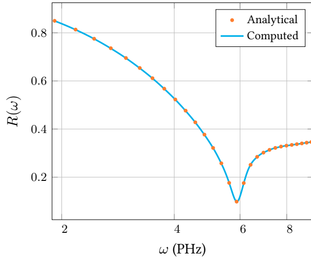
(b) Analytical and computed reflection spectra for a 4SOGP fit. As can be seen the DGT results are in good agreement with the analytical reflection coefficient. The results are similar for other dispersive models.
