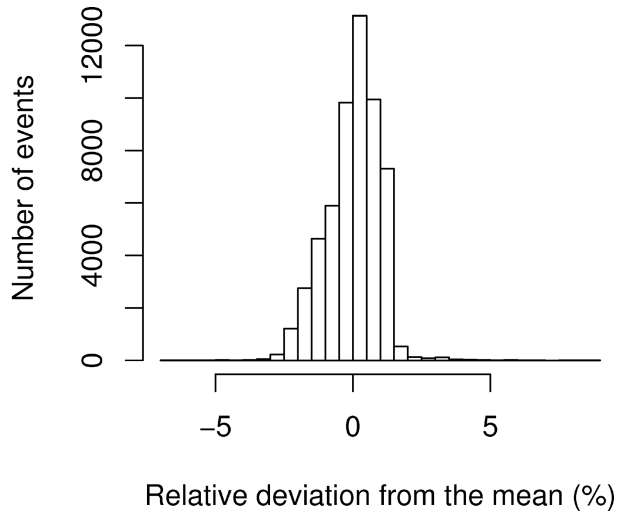
Fig. 3. Distribution of experimental noise.
