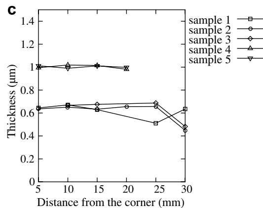
Fig. 9. Evolution of the refractive index and the film thickness along the diagonale of the two layer samples. (a) Refractive indices of the PZT and ZnO layers, (b) thicknesses of the ZnO layers, (c) thicknesses of the PZT layers.
