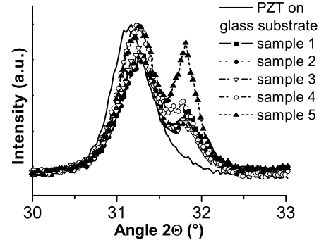
Fig. 10. X-ray diffraction diagrams.
