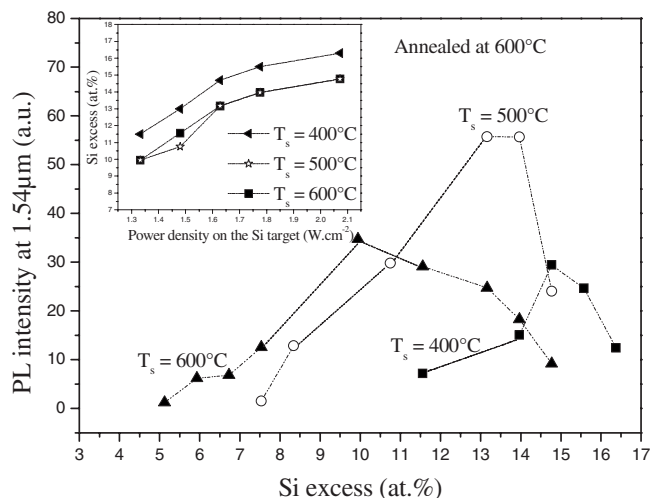
FIG. 5. Comparison of the variations of the Er PL intensity at 1.54 \mu\text{m} in function of Si excess, for the samples deposited at the indicated substrate temperatures and then annealed at 600^\circ\text{C} .
