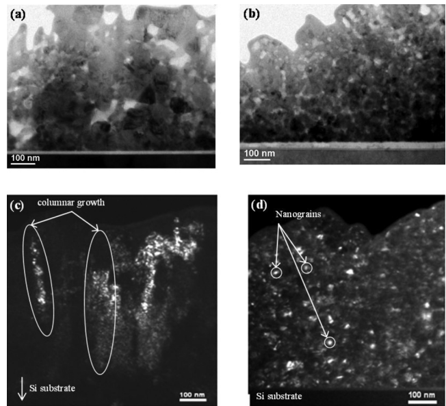
FIG. 1. Bright field TEM images of annealed samples elaborated with (a) r=9.7\% and (b) r=38.8\% . Dark field TEM images of the corresponding r values (c) and (d), respectively. In the first case, columnar growth and relatively large grains are observed whereas in the latter case, a random growth prevails with a concomitant nanostructuring of the film.
