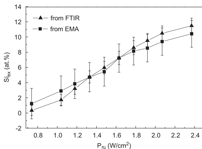
Fig. 2. Evolution of Si_{ex} (at.%) as a function of P_{Si} for as-deposited samples.
