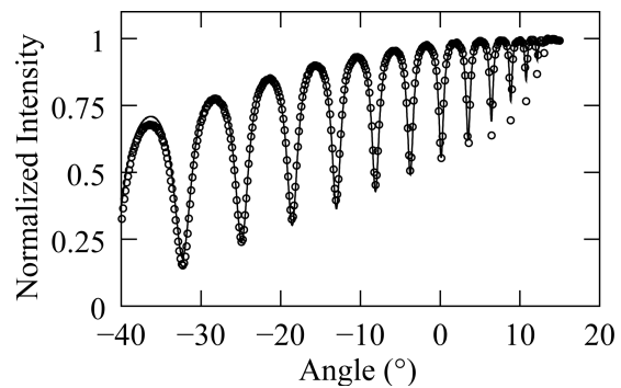
Fig. 4. Measured (O) and fitted (—) m -lines spectra of an S1818 film on silicon in TE mode.
