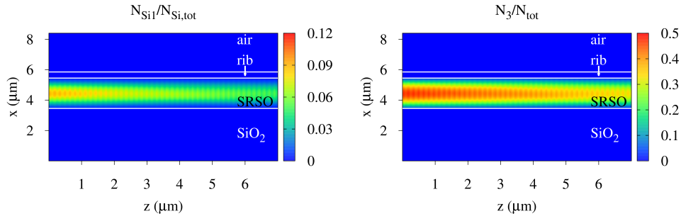
Fig. 9. Longitudinal section view of N_{Si}^*/N_{Si,tot} (on the left) and N_3/N_{tot} (on the right)
