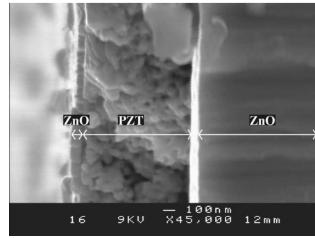
FIG. 10. SEM photograph of a three layer waveguide.
