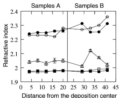
FIG. 13. Evolution of the refractive indices of the different layers of the three layer samples A_r , B_r ( n_1 : \square , n_2 : \circ , n_3 : \triangle ) and the two layer samples A_l , B_l ( n_1 : \blacksquare , n_2 : \bullet ).
