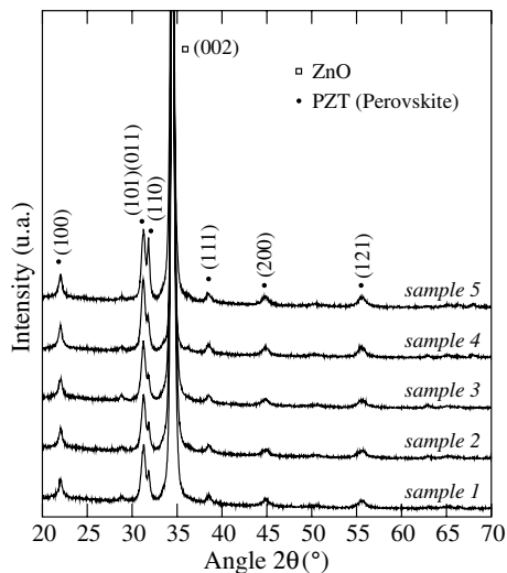
Fig. 6. X-ray diffraction diagram of the two layer films.
