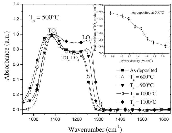
FIG. 1. Infrared absorption spectra of the layers deposited at T_s=500^\circ\text{C} , before and after annealing at the indicated annealing temperature T_a , as recorded at Brewster angle. The inset shows a typical shift of the TO 3 peak position for the as-grown sample at 500 °C, in function of the power density applied on the Si target.
