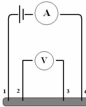
FIGURE 2.12: Four-points measurement of resistance
