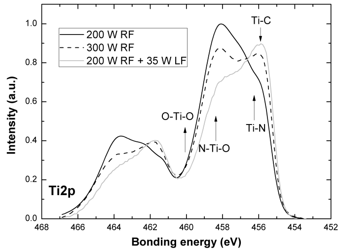
FIGURE 4.14: XPS Ti2p spectra of TiN samples
