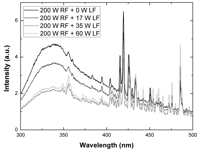
FIGURE 4.6: Impact of LF addition in Ar+H 2 OES in the 300 - 500 nm range
