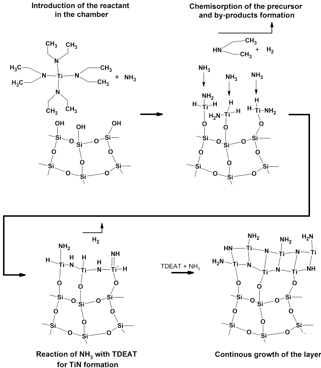
FIGURE 3.16: Possible reaction mechanism for deposition of TiN with TDEAT and NH 3 reactant gas.
