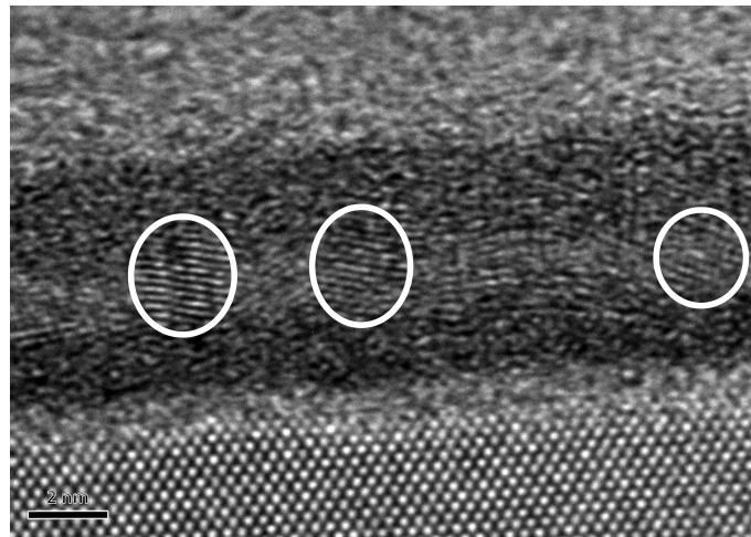
FIGURE 5.9: TEM observation of PEALD-TaCN/TiN/HfO 2 /SiO 2 /Si stack
