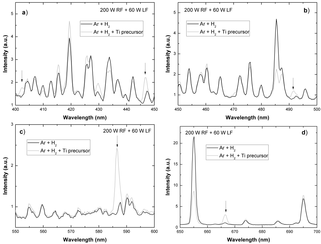
FIGURE 4.9: Effect of Ti precursor addition in the OES of the 200 W RF + 60 W LF plasma : a: 400 - 450 nm range; b: 450 - 500 nm range; c: 550 - 600 nm range ; d: 650 - 700 nm range
