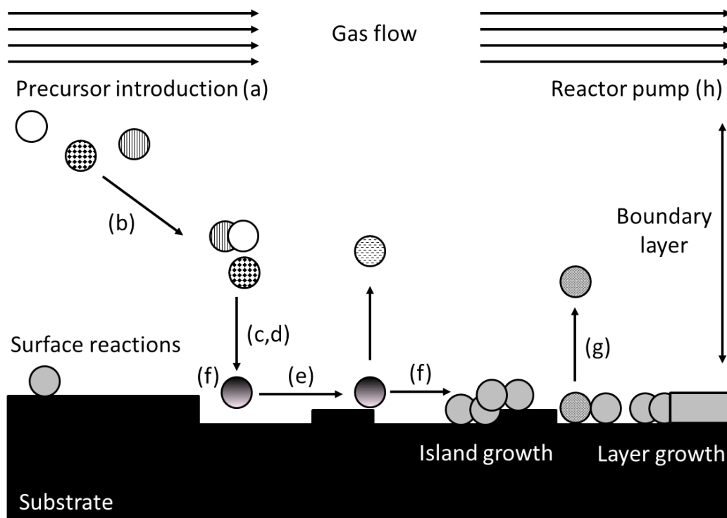
FIGURE 2.5: MOCVD reaction mechanisms
