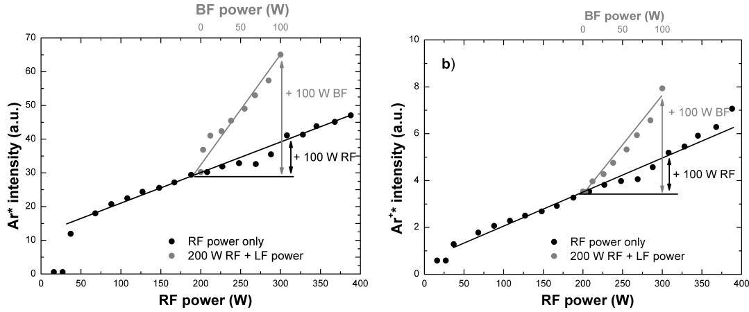
FIGURE 4.4: Evolution of the Ar^* (a) and Ar^{+*} (b) emission lines as a function of RF power and 200 W RF + LF power
