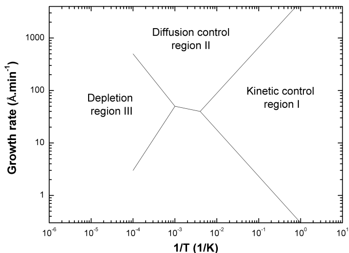
FIGURE 2.6: Film growth regimes for a CVD process
