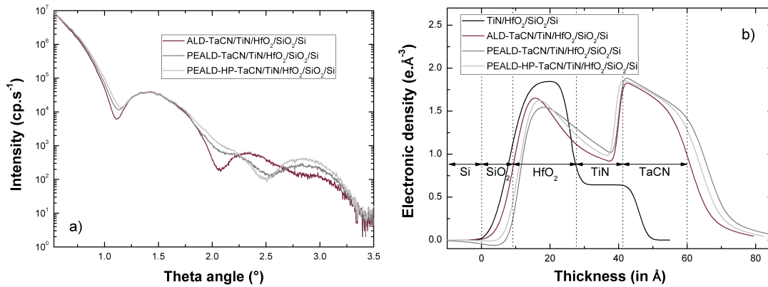
FIGURE 5.8: a : XRR spectra and b : electronic density extraction of ALD-TaCN/ \text{TiN}/\text{HfO}_2/\text{SiO}_2/\text{Si} , PEALD TaCN/ \text{TiN}/\text{HfO}_2/\text{SiO}_2/\text{Si} and PEALD HP TaCN/ \text{TiN}/\text{HfO}_2/\text{SiO}_2/\text{Si}
