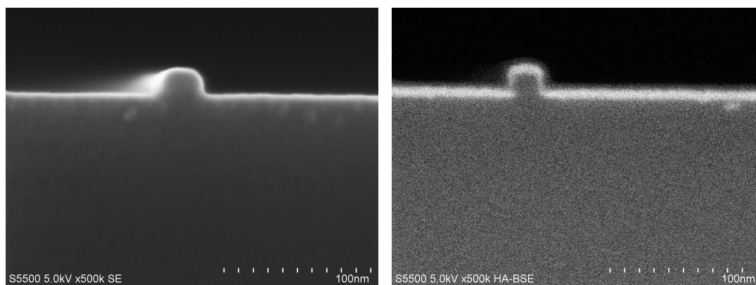
FIGURE 4.27: SEM observation of PEMOCVD deposited TaN on 15 nm Fin
