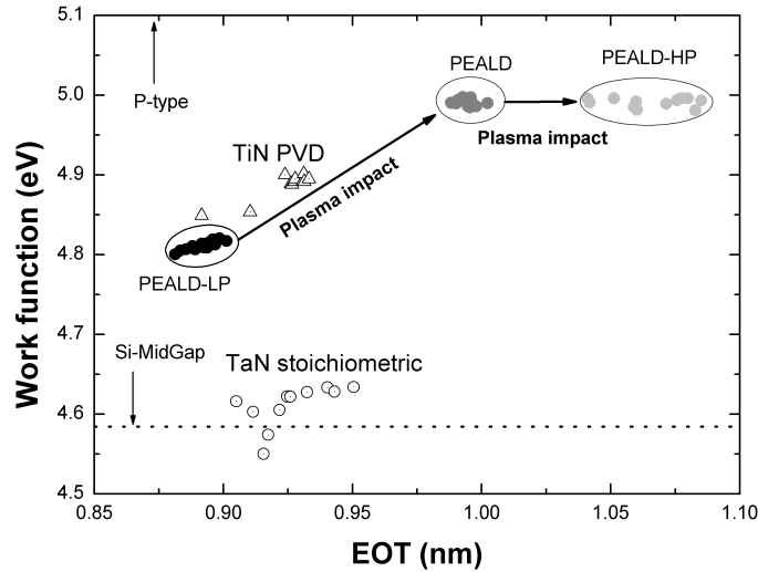
FIGURE 5.5: \Phi_m(\text{eff}) variation with TaCN plasma power increase
