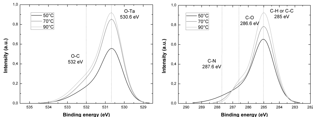
FIGURE 3.8: Evolution of O1s (left) and C1s (right) spectra in MOCVD TaN for different injector temperatures
