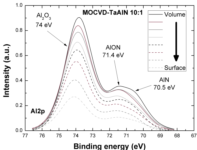
FIGURE 6.17: Evolution of Al chemical bonding from volume to extreme surface
