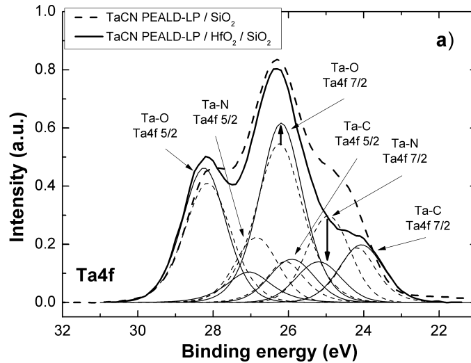
FIGURE 5.2: Comparison Ta4f XPS environment from PEALD-LP-TaCN/ SiO_2 / Si and PEALD-LP-TaCN/ HfO_2 / SiO_2 / Si
