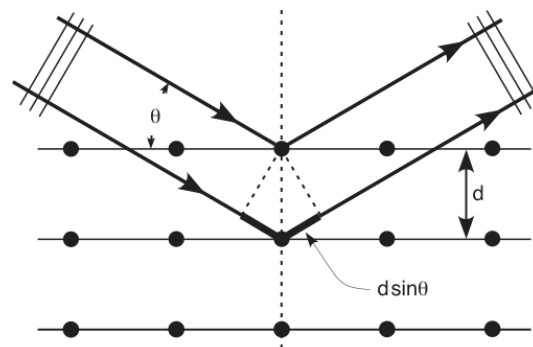
FIGURE 2.14: Schematic representation of interactions that result as an X-Ray beam hits a sample
