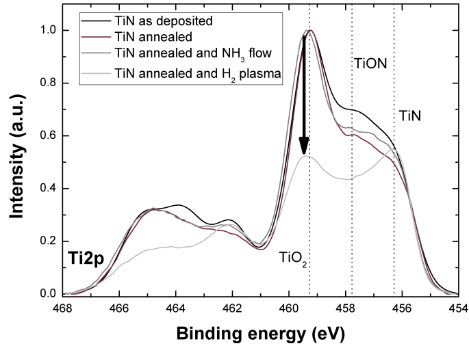
FIGURE 5.13: Ti2p XPS spectra of TiN as-deposited, after 325° C anneal, 325° C anneal with NH 3 flow, 325° C anneal with H 2 plasma
